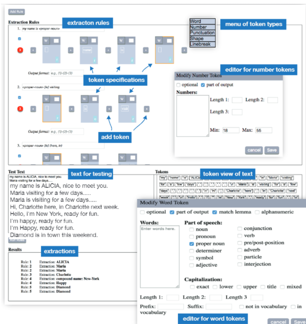
Figure 3: (Underlaid) The rule specification dashboard. (Overlaid) Configuration options for an atom that can be included in a larger rule template.
