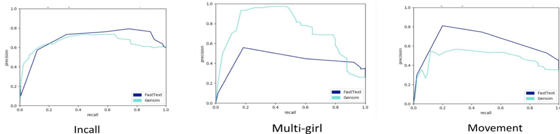
Figure 14: Precision-recall curves of the PV baseline ( gensim ) against Sim-ft ( fasttext ). Risky and Outcall (omitted herein) are qualitatively similar to Movement , with Sim-ft exhibiting a performance advantage.
