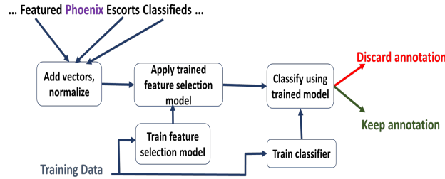
Figure 7: An illustration of supervised contextual classification on an example annotation (‘Phoenix’)
