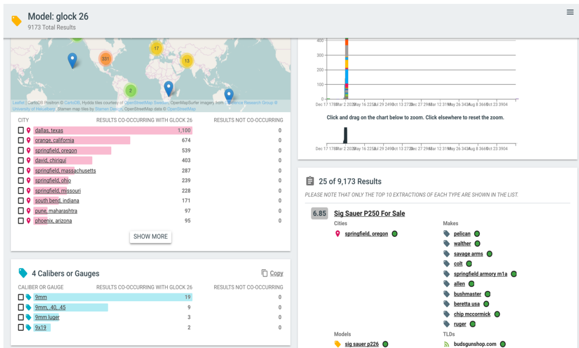
Figure 24: Entity-centric search (ECS) for the Illegal Firearms Sales domain in DIG.
