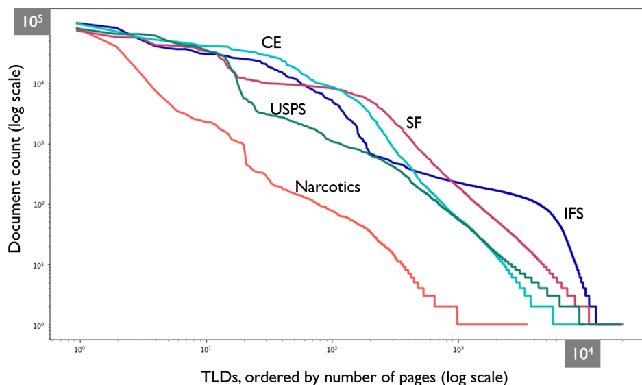
Figure 26: Document counts per TLD (Y-axis) against ranked list of TLDs (ordered by document count on X-axis).
