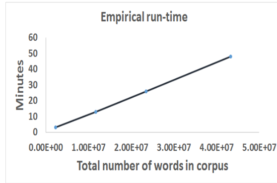
Figure 8: Empirical run-time of the adapted random indexing algorithm on the corpora in Table 4
