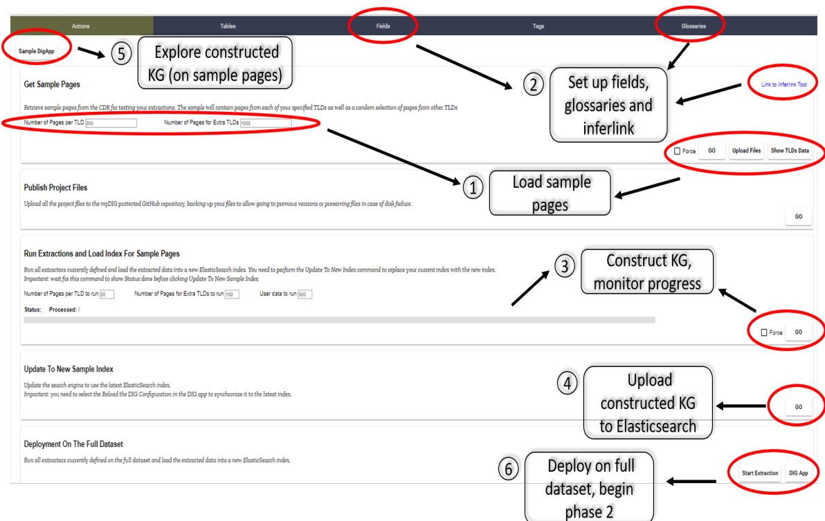
Figure 20: The DIG dashboard, with corresponding elements and actions.
