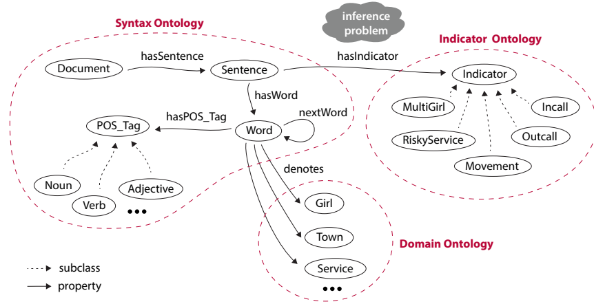
Figure 12: Ontologies for indicator mining.
