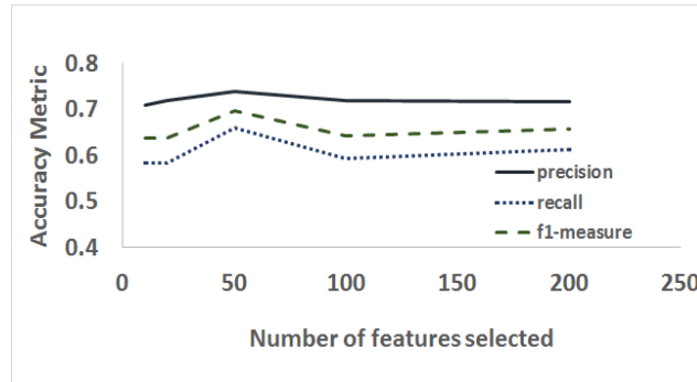
Figure 9: Effects of additional feature selection on the GT-Text-Name dataset (30% training data)
