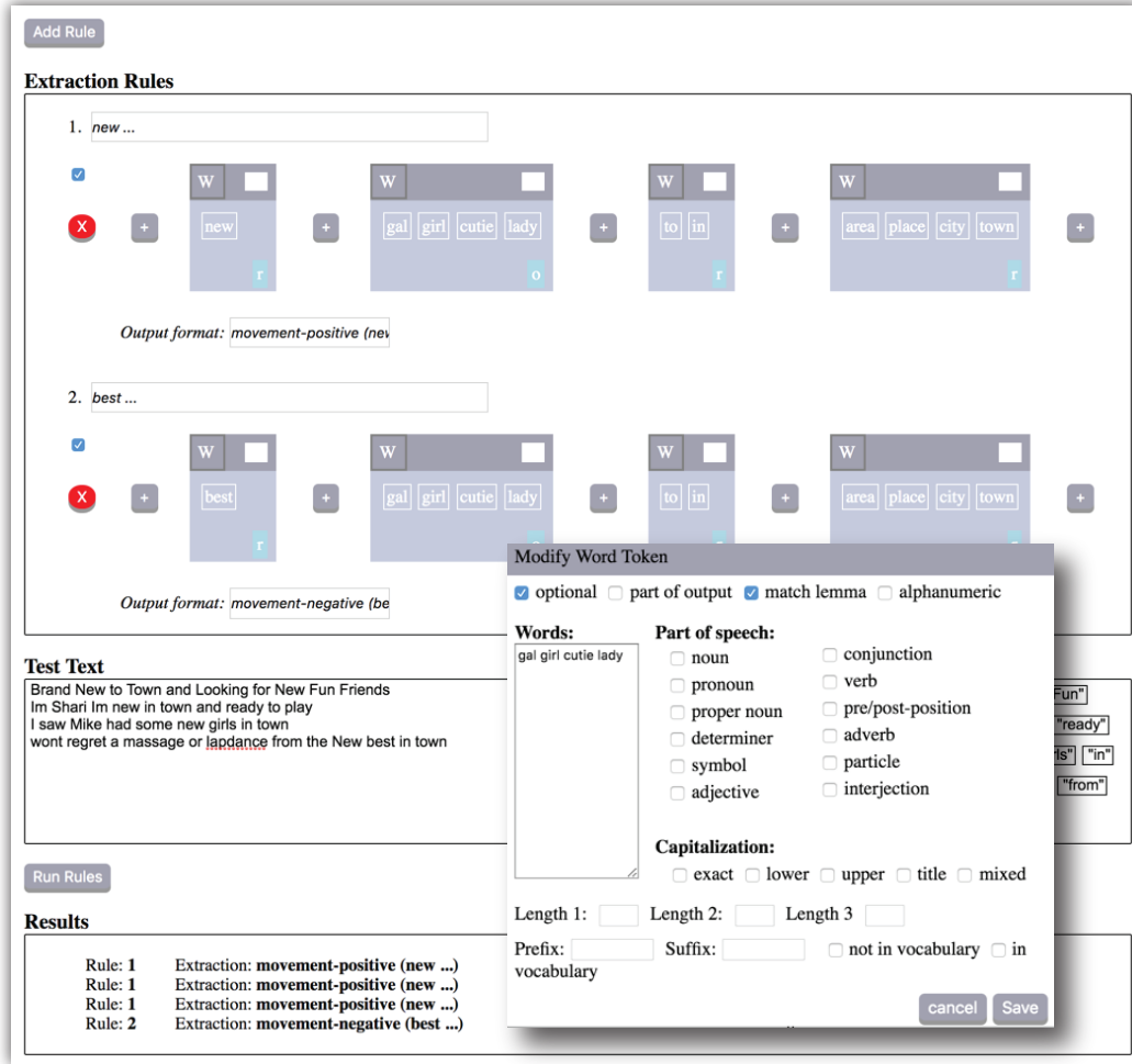
Figure 13: Easy to use interactive editor for defining indicator rules.
