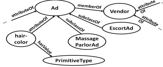
Figure 11: A fragment of the current investigative schema \mathcal{I} .
