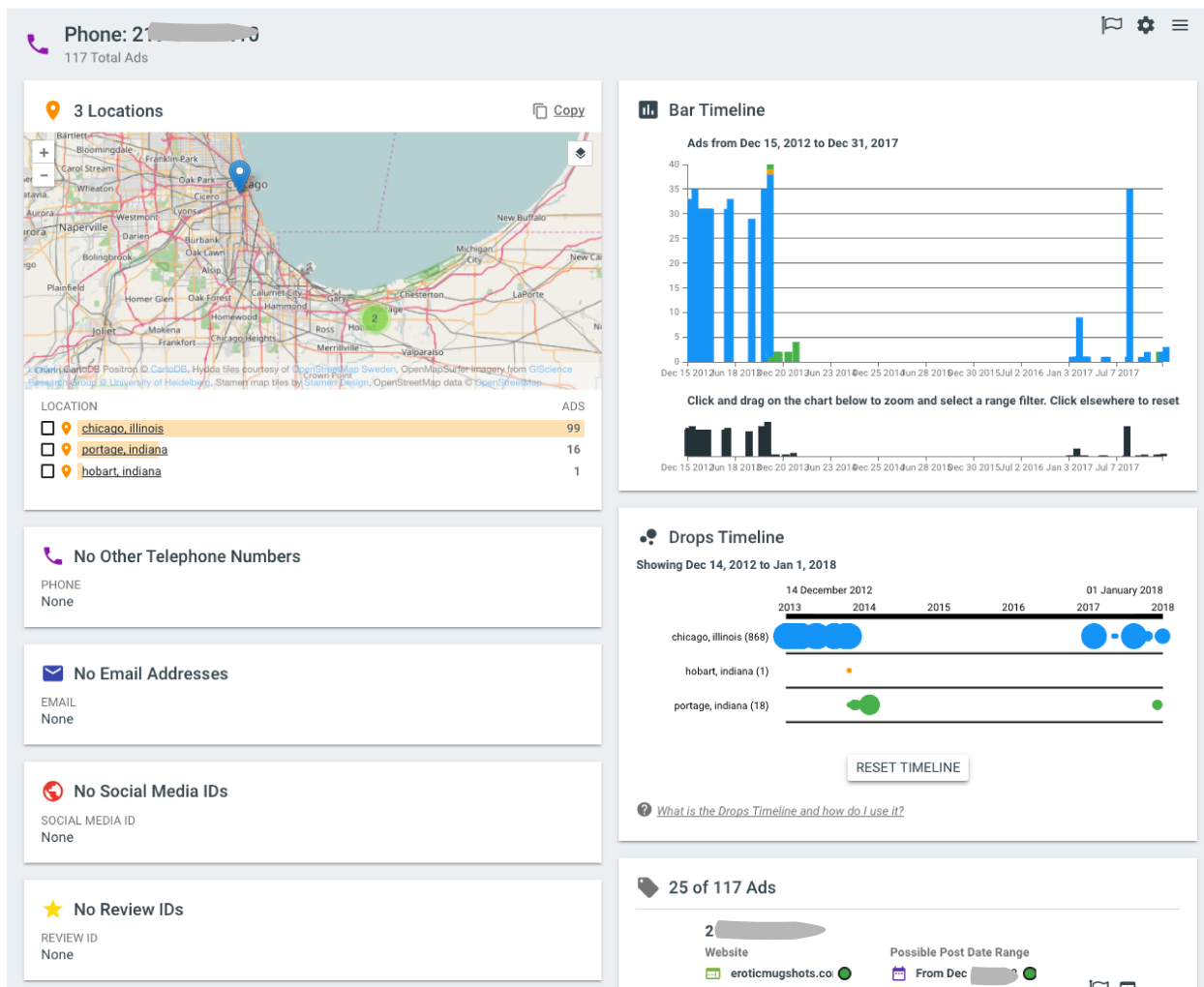
Figure 19: Continuing from Figure 18, the user is able to use entity-centric search facilities in DIG to collect a list of 117 ads, with details such as timelines and locations. These numbers can be used to conduct an investigation on the ground.
