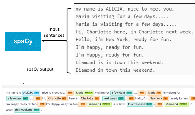
Figure 2: Input sentences from the online sex advertisement domain. Named entities were incorrectly extracted by pre-trained modules from SpaCy due to the unusual nature of the domain.
