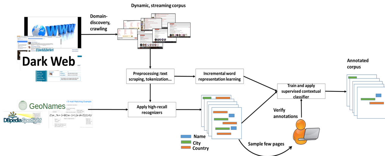
Figure 5: A high-level overview of the proposed information extraction approach
