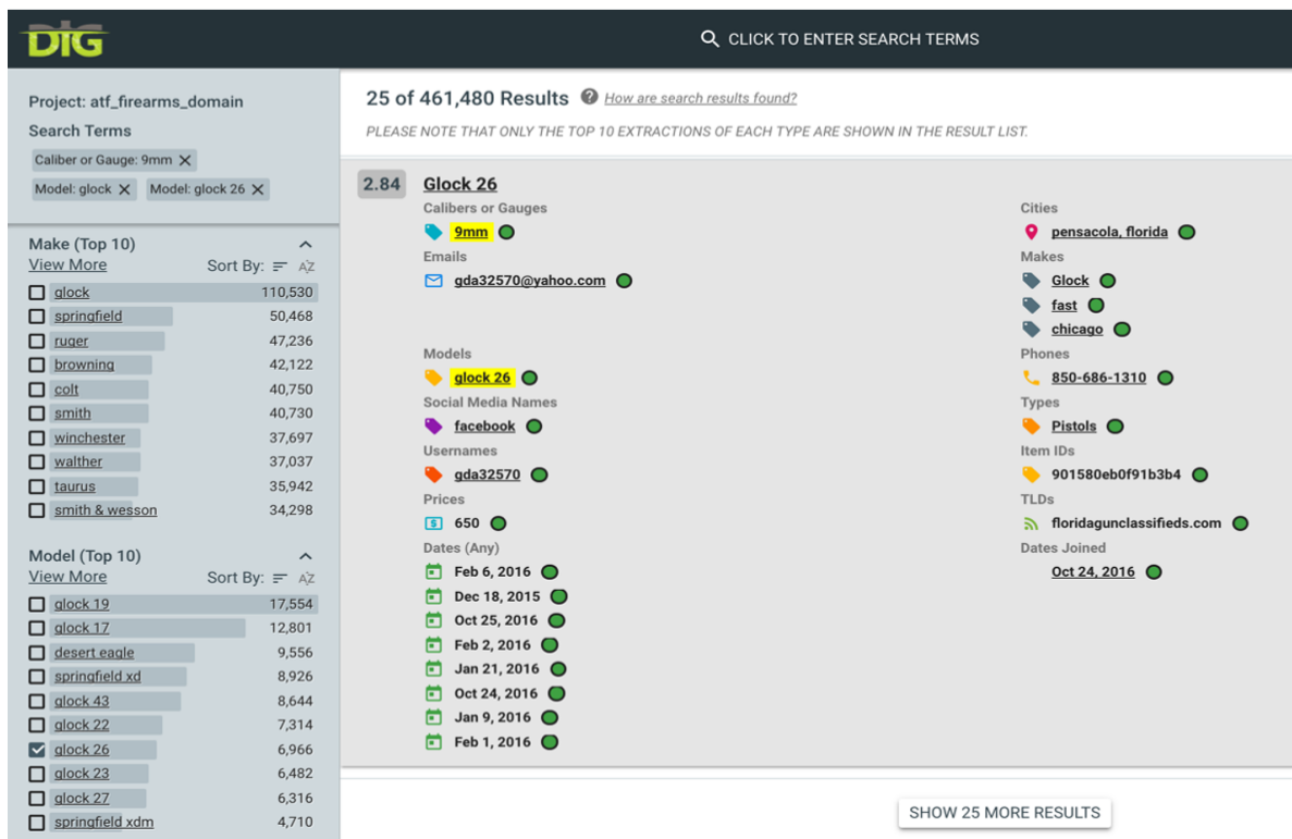
Figure 23: The search interface offered by DIG ( Illegal Firearms Sales domain).
