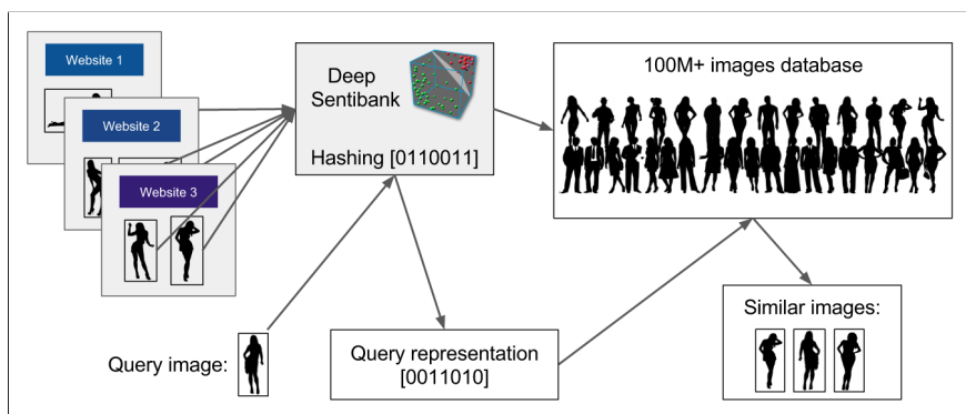
Figure 16: Overview of the Columbia Image Similarity Search tool.
