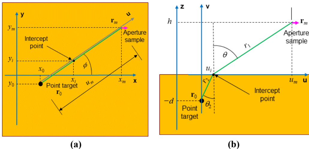
Fig. A-1 Geometry involved in the propagation path (green line) between radar and target consistent with Snell's law: a) top view and b) side view in the u-v plane. Note that v is the vertical axis going through the point target.
