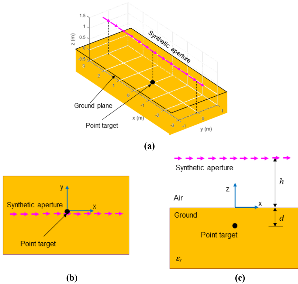
Fig. 4 GPR SAR system using a linear synthetic aperture in down-looking configuration: a) perspective view, b) top view, and c) side view
