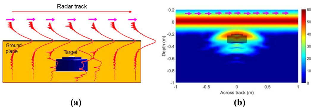
Fig. 1 B-scan radar mapping technique in down-looking GPR: a) schematic representation of the scanning principle and b) actual B-scan of a buried landmine obtained by AFDTD computer simulation
