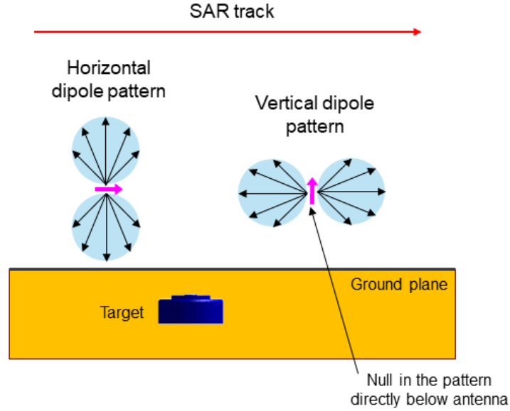
Fig. 3 Dipole antenna patterns in a GPR SAR system for horizontal and vertical dipole orientations
