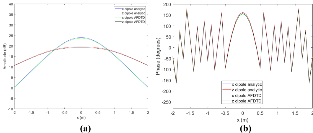
Fig. 8 Comparison of the PTR as a function of position along the synthetic aperture, computed by the analytic formulas and AFDTD simulations for side-looking configuration: a) magnitude in decibels and b) phase in degrees
