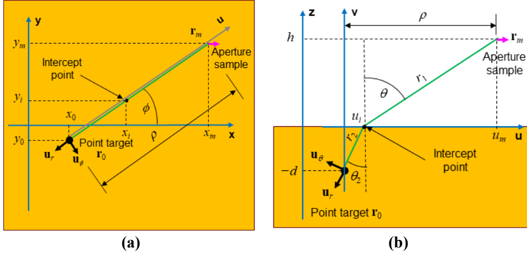
Fig. 6 Geometry involved in the propagation path (green line) between radar and target consistent with the Green's function asymptotic expansion: a) top view and b) side view in the u - v plane. Note that v is the vertical axis going through the point target.
