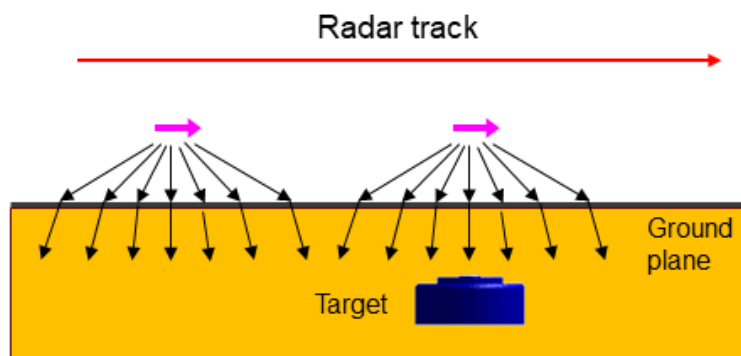
Fig. 2 Schematic representation of a GPR system with the dipole antenna placed close to the ground, showing the self-focusing effect of the beam upon propagation into the ground
