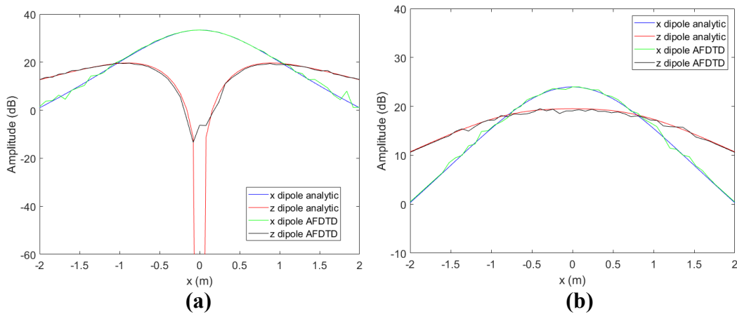
Fig. 10 Comparison of the PTR as a function of position along the synthetic aperture, computed by the analytic formulas and AFDTD simulations of scattering by a metallic sphere: a) down-looking configuration and b) side-looking configuration
