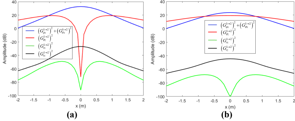
Fig. 9 Comparison of various components of the PTR as a function of position along the synthetic aperture, computed by AFDTD simulation: a) down-looking configuration and b) side-looking configuration
