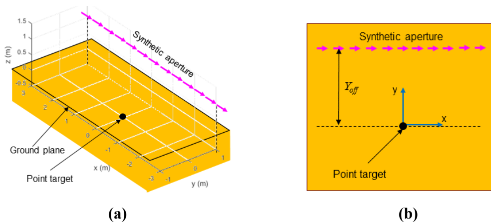
Fig. 5 GPR SAR system using a linear synthetic aperture in side-looking configuration: a) perspective view and b) top view
