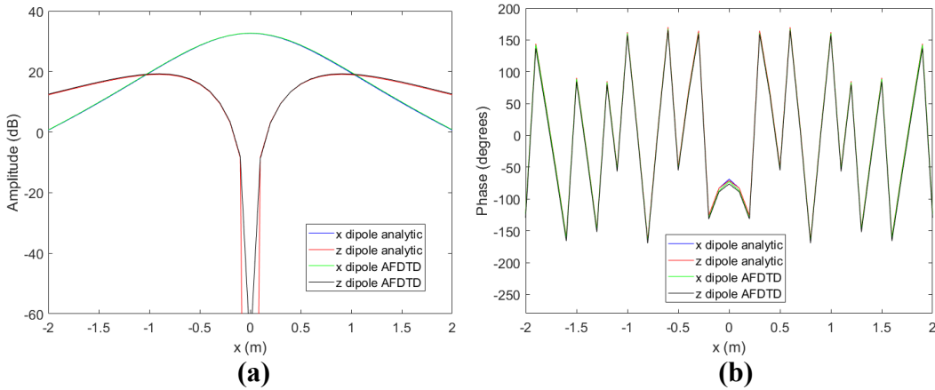
Fig. 7 Comparison of the PTR as a function of position along the synthetic aperture, computed by the analytic formulas and AFDTD simulations for down-looking configuration: a) magnitude in decibels and b) phase in degrees
