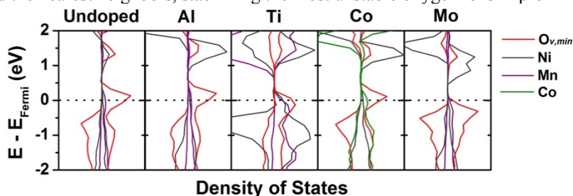
Figure 1.5: Projected density of states of the least stable oxygen ion and the nearest cations show Mo-doped material stabilizes the least stable oxygen ion by shifting bonding levels beneath the Fermi energy.
