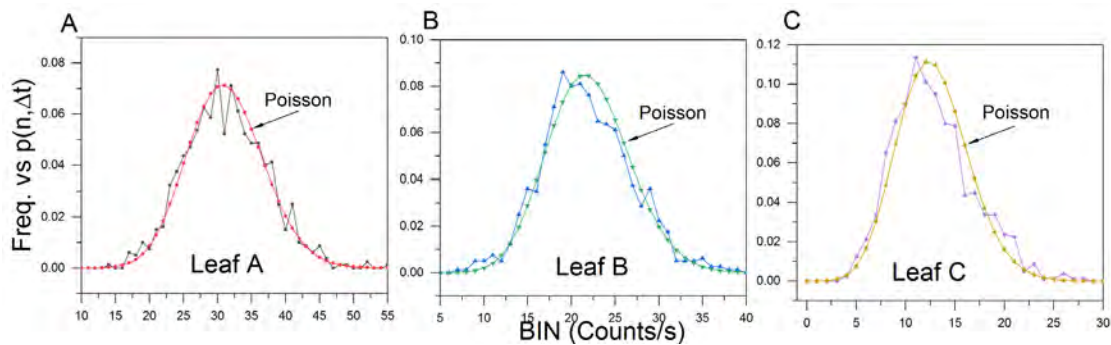
Aerobic photocount observed frequencies vs. Poisson predicted distributions (leaves A-C) of the hyperbolic decay data (last 800 s). Observed photon count frequencies closely approximate a Poisson predicted distribution ( \mu_A = 31.25 ; \mu_B = 22.03 and \mu_C = 12.82 ).
