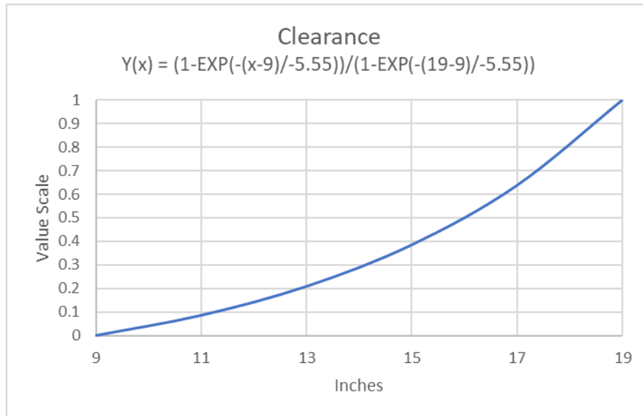
Figure 10. Value Graph of Ground Clearance
