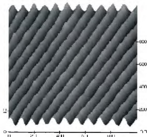
Figure V-9. Magnified Atomic Force Micrograph. An "egg-carton" pattern on the surface of an electropolished aluminum surface. The pattern was produced after polishing for 30 seconds using techniques routinely used by the anodizing industry.
