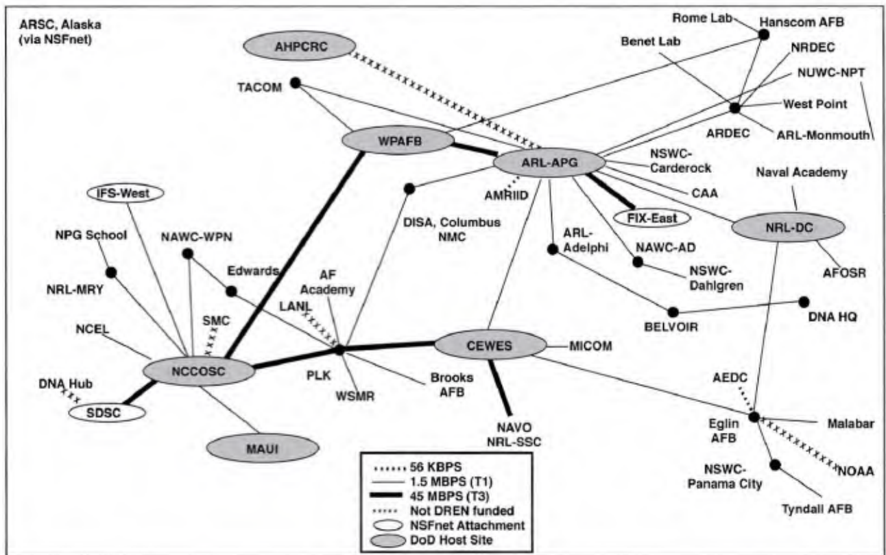
Figure IV-6. IDREN Configuration
