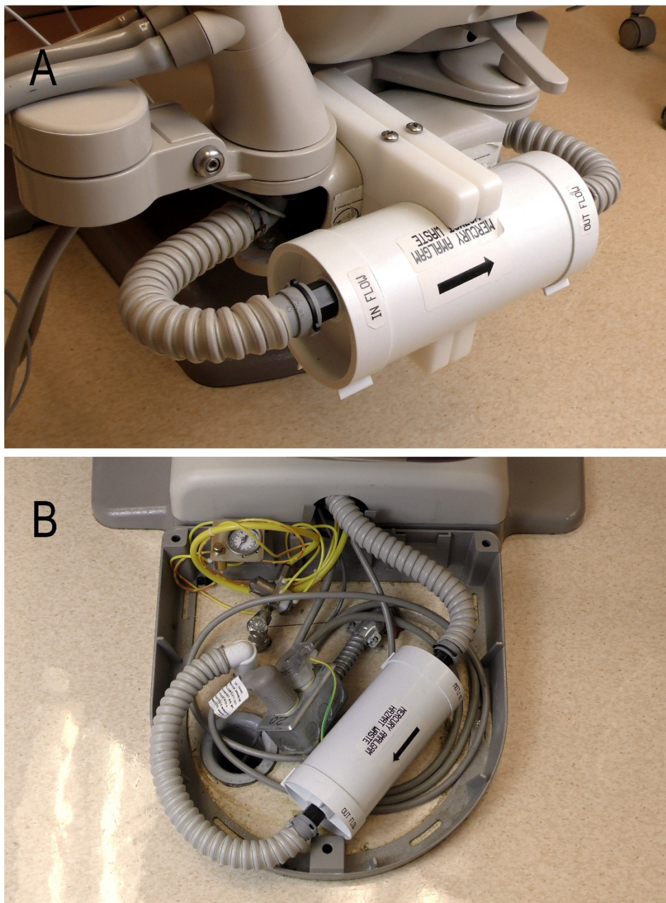
Figure 2. A typical installation of the DD2011P chairside amalgam separator (white cylinder) on the rear support link of an A-Dec 500-Series dental chair ( A ). This particular installation makes use of the optional mounting brackets (white clamps with screws). An alternative installation is shown ( B ) in which the separator is contained within the floor box under the chair. Both installations illustrate the use of the quick-disconnect fittings (black).
