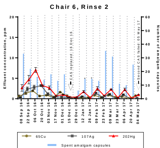
Figure 6. Samples of effluent were collected from installed amalgam separators and analyzed for mercury, silver, and copper. Concentrations (ppm) of each metal are shown (reference the left Y-axis), juxtaposed against the number of spent amalgam capsules collected from the corresponding chair during the corresponding period (blue bars, reference the right Y-axis).
