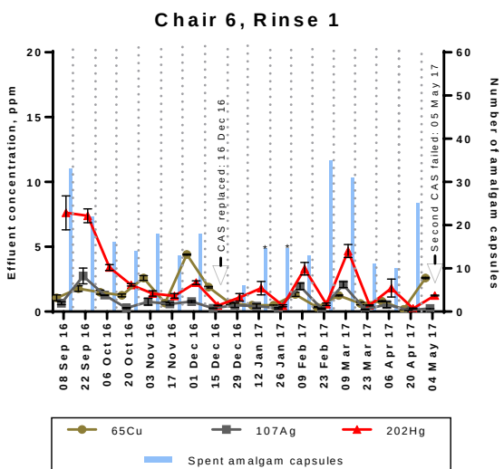
Figure 6. Samples of effluent were collected from installed amalgam separators and analyzed for mercury, silver, and copper. Concentrations (ppm) of each metal are shown (reference the left Y-axis), juxtaposed against the number of spent amalgam capsules collected from the corresponding chair during the corresponding period (blue bars, reference the right Y-axis).
