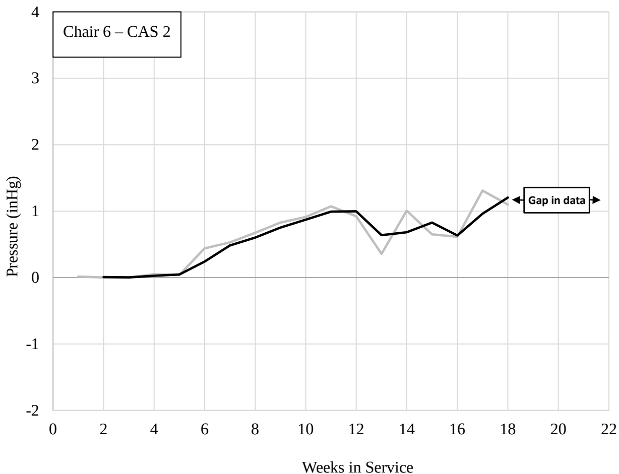
Figure 9. Timelines of pressure sensor differential during amalgam separators' service lives. Moving averages were calculated from data collected during working hours. For each chair, the averages of the preceding week's data, analyzed at weekly intervals, are displayed as gray lines. Similarly, the averages of the preceding two weeks' data for each chair, analyzed at weekly intervals, are displayed as black lines. A loose sensor wire caused data drop-out for Chair 4, CAS 2 (4.2) in the 1-10 week period. Chair 6, CAS 2 (6.2) data were corrupted for the last four weeks of the recording. The other seven pressure data timelines run the complete service life from installation to replacement.
