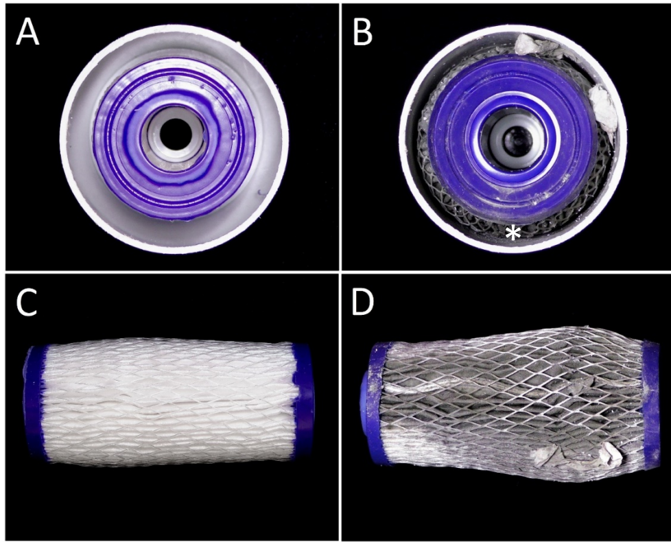
Figure 7. Representative cross-sectional and interior views of a DD2011P CAS before installation and at the end of its service life. Panel (A) : Cross-sectional view of a DD2011P CAS before installation. Panel (B) : Cross sectional view of the CAS at the end of service life. Note the minimal amount of accumulated sediment (white asterick) within the interior space between the filter element and the plastic filter housing. Panel (C) shows the interior filter medium removed from a new DD2011P CAS unit. Panel (D) shows the same filter medium removed from a CAS at the end of its service life.
