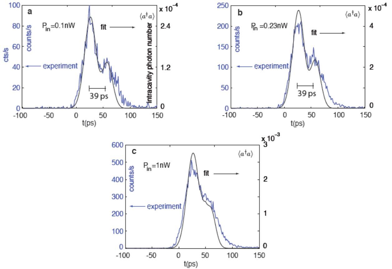
Figure 3. Time-resolved reflectivity measurement shows Rabi oscillation frequency g/2\pi = 29 GHz. We show three excitation powers A) , B) , C) . The observations are fit with a full master equation model; in all three plots, the photon flux into the cavity is scaled equally from the measured incident power (0.1 nW, 0.23 nW, 1 nW before the lens).
