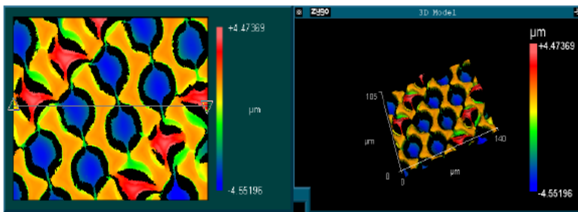
Figure 7. Convex non-axisymmetric shells co-existing with concave axisymmetric shells in a surface of polymethylmethacrylate- b -poly( n -butyl acrylate)- b -polymethylmethacrylate triblock copolymer. Left image displays 2-d contour map of surface. Right image is 3-d projection of surface topography.
