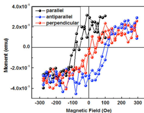
Figure 2. Magnetization curves for a permalloy layer that is exchange coupled to an underlying BFO film as a function of the direction of the electric field applied to the underlying BFO layer.
