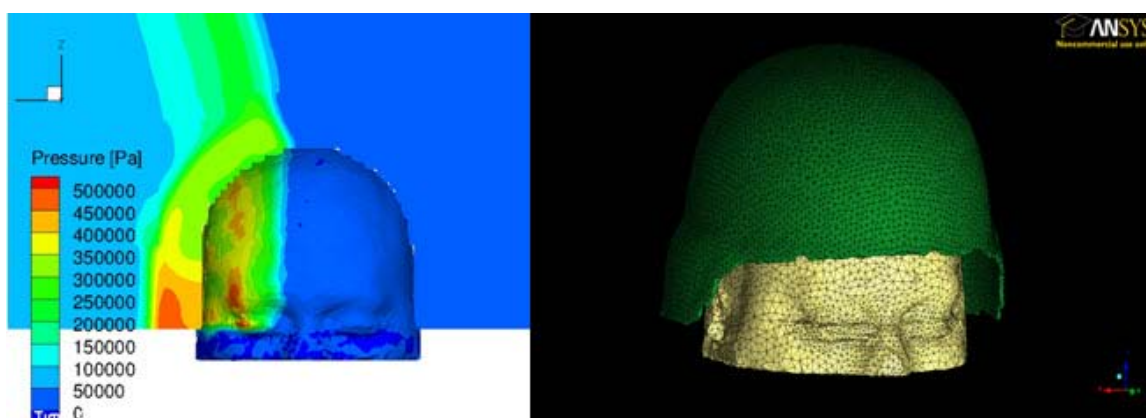
Figure 3. (a) Blast simulation showing a snapshot of pressure distribution from a side detonation (b) meshed head with Advanced Combat Helmet (ACH).
