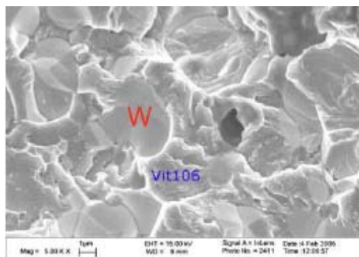
Figure 11. SEM image showing fracture surface of W-Vitreloy106 composite.
