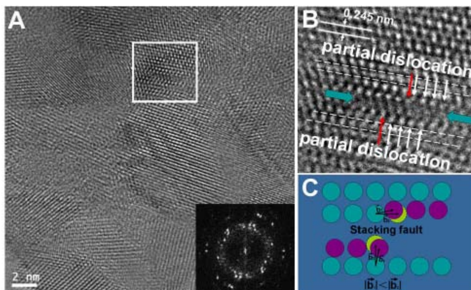
Figure 3. HRTEM image and electron diffraction pattern of the impact compressed nacre. (A) Partial dislocations as indicated by the white box. The insert is the diffraction pattern from the HRTEM image. (B) Partial dislocations with stacking faults. (C) Schematic analysis.
