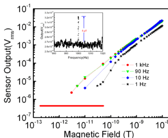
Figure 4. MR sensor output at different frequencies as a function of field strength.
