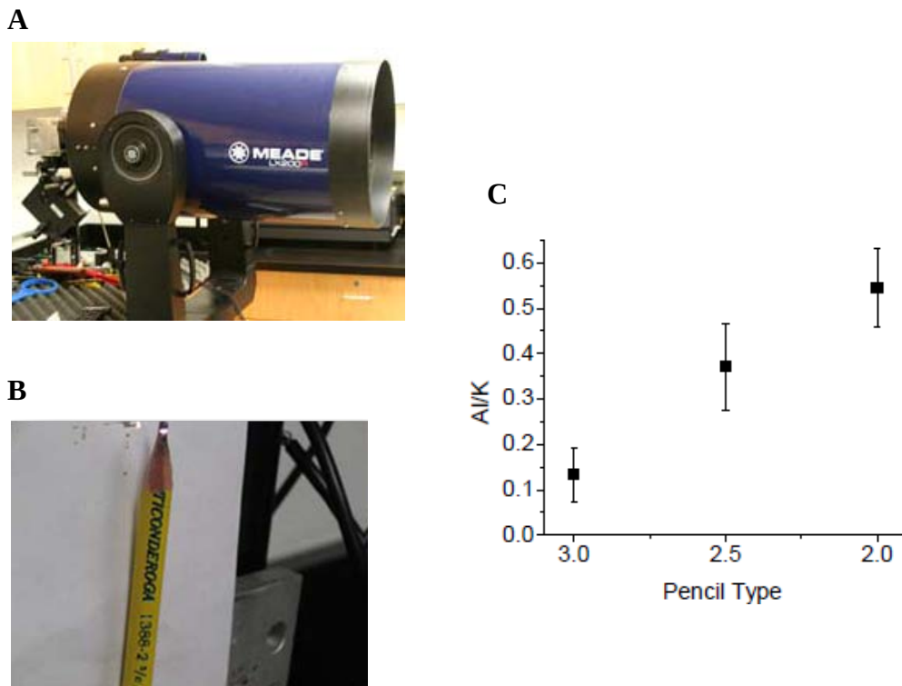
Figure 9. Demonstration of potential for femtosecond laser desorption of molecules to detect improvised explosive devices: (A) A Meade telescope is used to collect backscattered emission off of (B) a #2.5 pencil. There are two types of clay in the pencils: Illite ( \text{K}_{0.6}(\text{H}_3\text{O})_{0.4}\text{Al}_{1.3}\text{Mg}_{0.3}\text{Fe}_{0.1}\text{Si}_{3.5}\text{O}_{10}(\text{OH})_2(\text{H}_2\text{O}) ) and Kaolinite ( \text{Al}_2\text{Si}_2\text{O}_5(\text{OH})_4 ), in different proportions, and (C) analysis of IBS ratio of Al/K revealed the variation of clay composition among individual pencils.
