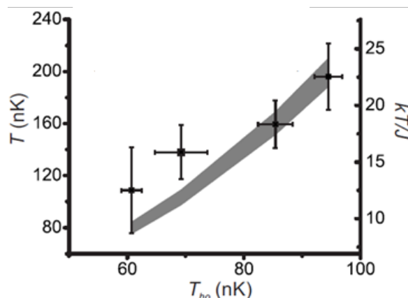
Figure 7. Temperature (y-axis) obtained by measuring the in-lattice size of the gas, the latter mapped onto its corresponding free gas temperature (x-axis): these data were obtained using the measurement of the gas cloud size for an optical lattice with a lattice depth at which the first method is inadequate. The shaded grey region is the theoretically expected temperature for the system.
