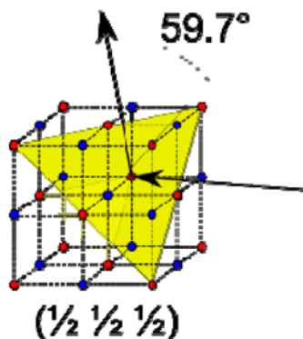
Figure 12. Bragg scattering of light off a plane of like magnetic moments (yellow triangle). The lattice will be a standing wave of light with ^6\text{Li} atoms in the valleys of the standing wave. Ordering results from interactions between the atoms at different sites.
