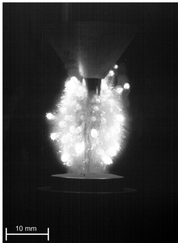
Figure 4. Still image taken from a high speed video showing ignition of individual particles within the Mg cloud aerosolized by the spark shockwave which results in a bright white flame.
