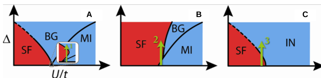
Figure 11. Three diagrams proposed to represent DBH model: phase diagrams (A), (B), and (C) were each proposed to represent the DBH model but provide mutually-conflicting descriptions. The phase diagrams show four phases: superfluid (SF), Bose glass (BG), Mott insulator (MI), and insulator (IN) as a function of the disorder strength ( \Delta ), and the ratio of on-site interaction strength to the energy required for an atom to hop from one site to the next ( U/t ). Researchers funded through ARL/ARO have ruled out model B, but the remaining models will be tested in FY09.
