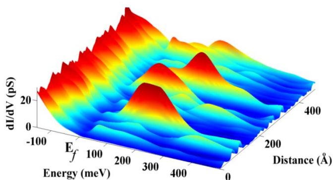
Figure 8. Spatial distribution of the electronic states of Ga 0.95 Mn 0.05 As near the Fermi Energy
