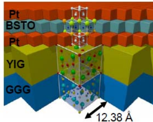
Figure 1. Illustration of the cube-on-cube layering of the YIG-Pt-BSTO (Barium Strontium Titanate)-Pt heterostructure: notice the tight “sandwiching” of the components, which allows for a more efficient coupling of their individual properties than any previous structures. [Das et al., 2009]
