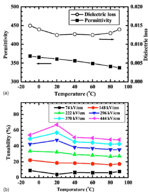
Figure 10. (a) Dielectric permittivity and dielectric loss of BST multilayer films as a function of operation temperature; (b) Temperature dependence of tunability as a function of external electric field.
