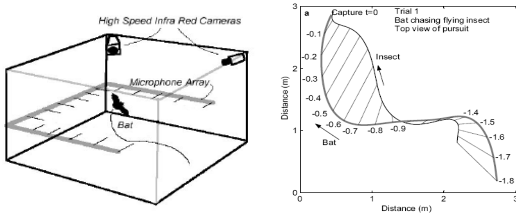
Figure 4. Echolocating bats use a nearly time-optimal strategy to intercept prey.
