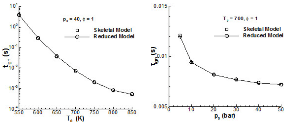
Figure 6. N-heptane ignition times predicted using reduction concept in conjunction with the LLNL tabular information and with a slope adjustment for the initial enthalpy increase due to the heavy species reaction (lines).
