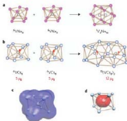
Figure 9. Lowest energy structures of V_2Na_{16} and (VCs_8)_2 dimer. Total and net spin electron density of VCs_8 . a, V_2Na_{16} and b, (VCs_8)_2 dimer starting from free clusters. The arrows indicate the direction of the V local spin moments. The superscripts indicate spin multiplicity. The total electron density c, and net spin electron density d (isovalue = 0.001 a.u.), in a VCs_8 cluster. The spin density is mostly localized at the center around the V-site.
