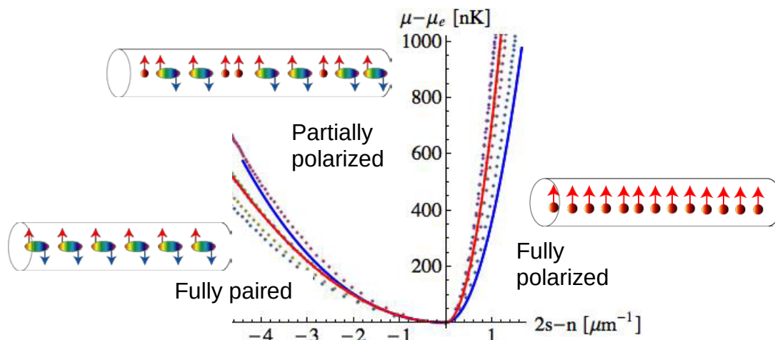
Figure 8. Agreement between experimental and theoretical phase diagrams for the one dimensional Fermi gas: dotted lines indicate experimental data and the red line their average, while the blue line is the theoretical calculation.
