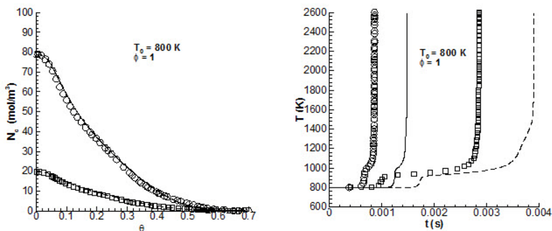
Figure 5. Comparisons between the n-heptane oxidation predictions of the LLNL skeletal model using Chemkin II (symbols) and reduced model in conjunction with LLNL tabular information (lines).
