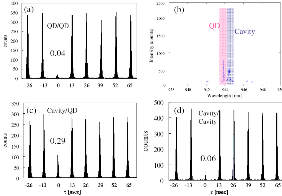
Figure 4. Auto- and cross-correlation measurements of the PC cavity emission: (A) The plot displays a photon auto correlation histogram of the QD emission. The QD peak wavelength is selected by a grating. (B) The PL spectrum for cross correlation measurement is shown, followed by (C), the cross-correlation measurement of QD and (D), and the auto correlation measurement of the cavity peak in (B). The cavity peak is strongly anti-bunched, so the cavity can be used for collection of output photons when QD is resonantly excited.
