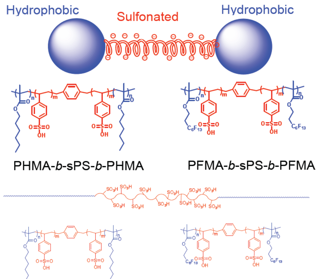
Figure 1. Midblock sulfonated triblock copolymers: researchers successfully integrated a sulfonated middle block in these polymers, surrounded by the hydrophobic (water-repelling) subunits on either side. These sulfonated middle blocks that can be used to tune the level of sulfonation in the entire polymer, thereby providing a method for modulating the transport of these polymers in a variety of solutions.
