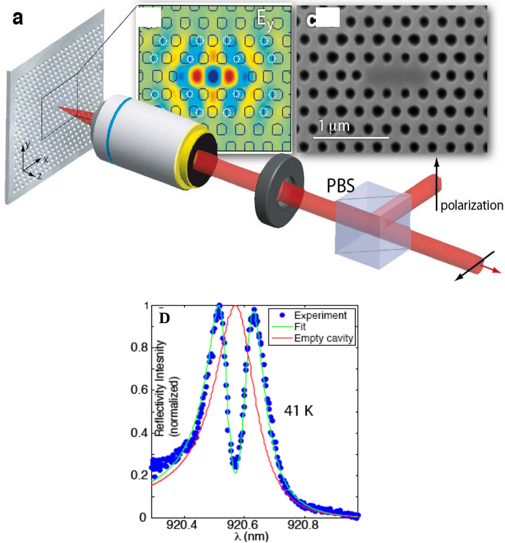
Figure 2. Experimentation for achieving quantum dots in crystal resonators: (A) results from this laboratory were obtained using this cross-polarized confocal microscope setup. (B) The E_y field in the L3-cavity structure illustrating how the structure is perturbed, at the sites indicated by dashed circles to increase output coupling. (C) The structure was characterized in part with a scanning electron micrograph. (D) Vacuum Rabi splitting is illustrated, as observed in the reflectivity from the strongly coupled QD/cavity system. For comparison, we show the reflectivity of an empty cavity.
