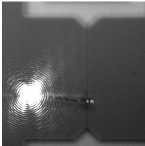
Figure 9. Hybrid Nanowire Device Exhibiting Rescattering-Based Plasmon Propagation.
