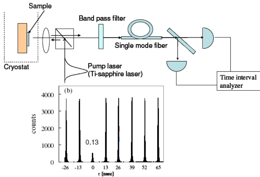
Figure 5. Fiber coupling experiment: (A) The HBT setup with fiber coupling uses only a band pass filter to reject the pump beam; (B) histogram of single photon with fiber coupling.
