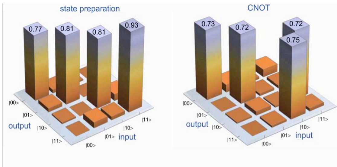
Figure 6. Experimental truth table of a neutral atom CNOT gate: the probabilities of state preparation are shown on the left and for the CNOT gate on the right.
