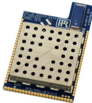
Figure 1. OE3x Module
