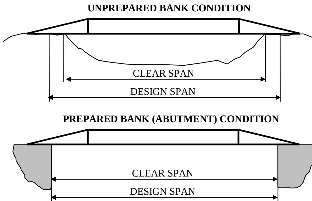
FIGURE 2-1: Bridge Spans
