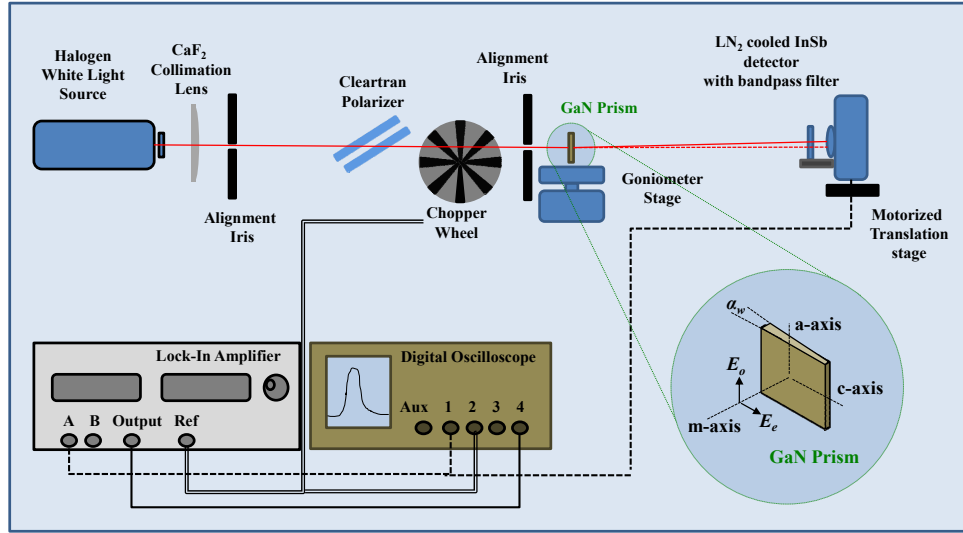
Fig. 2. Schematic of the experimental setup used to measure the chromatic dispersion of bulk GaN crystal. Inset shows orientation of GaN prism and directions of ordinary, E_o , and extraordinary, E_e , polarizations.
