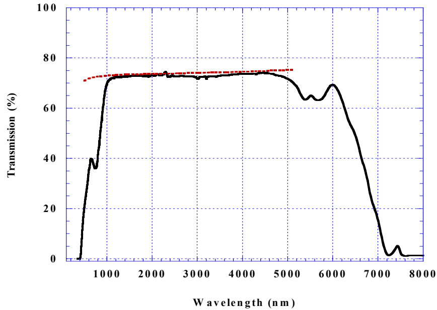
Fig. 1. Room temperature transmission of a semi-insulating GaN m-plane wafer 0.91 mm thick. Dotted line shows the calculated Fresnel losses based on the reported Sellmeier equations.
