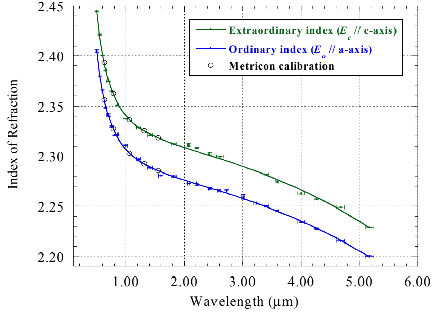
Fig. 3. Room temperature measurements of the refractive index of bulk GaN. Error bars and Metricon calibration points are discussed in the text. The solid curves are the best fit two-term Sellmeier Eqs. (2) and (3).
