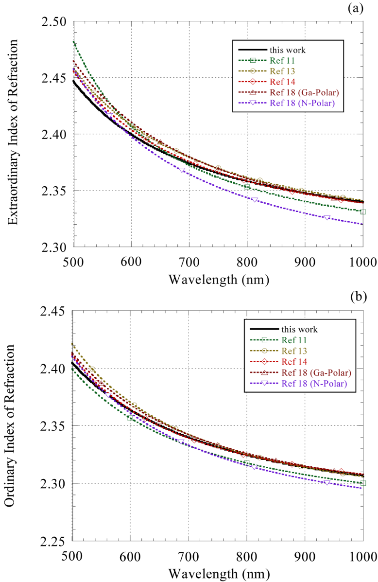
Fig. 4. Comparison of visible and near-IR Sellmeier fits of the extraordinary and ordinary refractive index of GaN.
