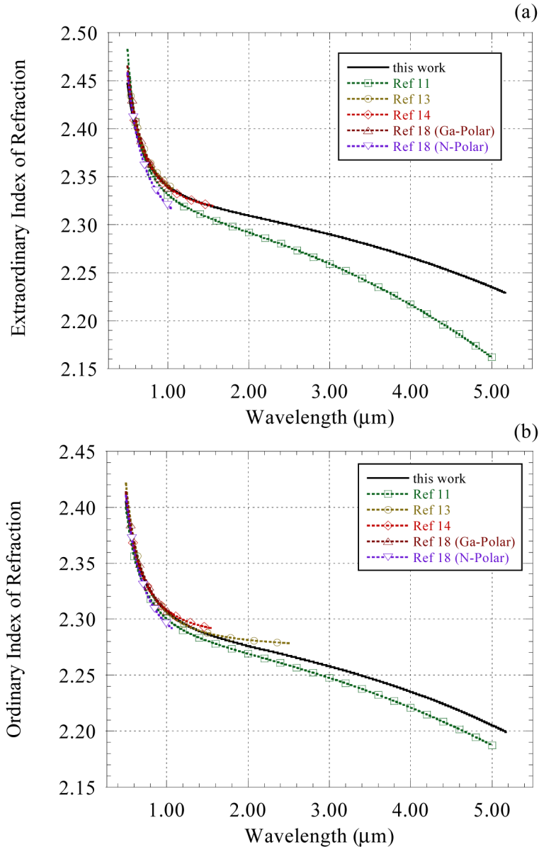
Fig. 5. Comparison of mid-IR Sellmeier fits of the extraordinary and ordinary refractive index of GaN.
