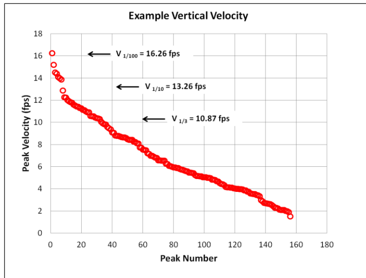
Figure B5. Impact Velocity Sorted Largest to Smallest
