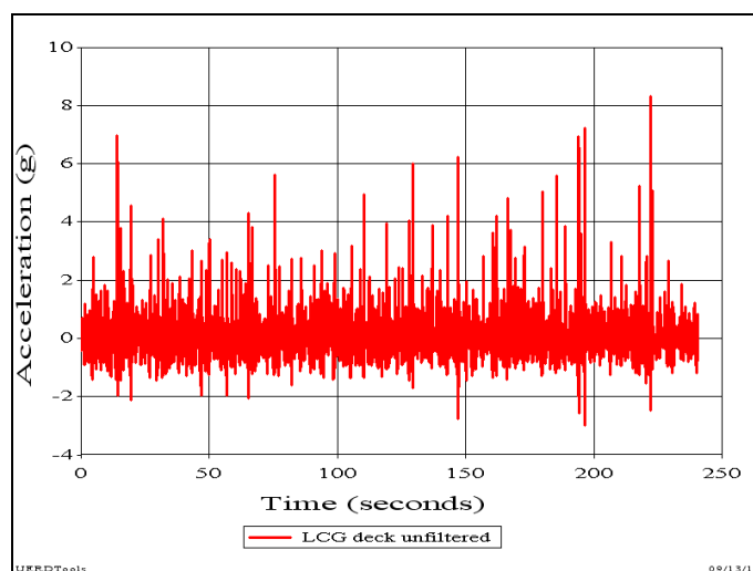
Figure A2. Acceleration in Units of “g”
