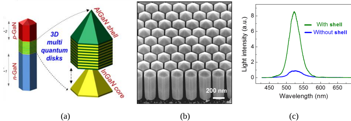
Figure 2. (a) Schematic of InGaN/AlGaN nanowire heterostructure, which consists of n -GaN cladding layer, core-shell InGaN/AlGaN multiple quantum disk active region, and p -GaN cladding layer. (b) Tilted-view SEM image of the InGaN nanowires. (c) Photoluminescence emission spectra of InGaN/AlGaN core-shell multi-quantum disk nanowires (green curve) and InGaN/GaN multi-quantum disk nanowires without AlGaN shell (blue curve) measured at 300 K.
