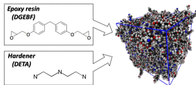
Fig. 1. Schematic of neat epoxy unit cell.
