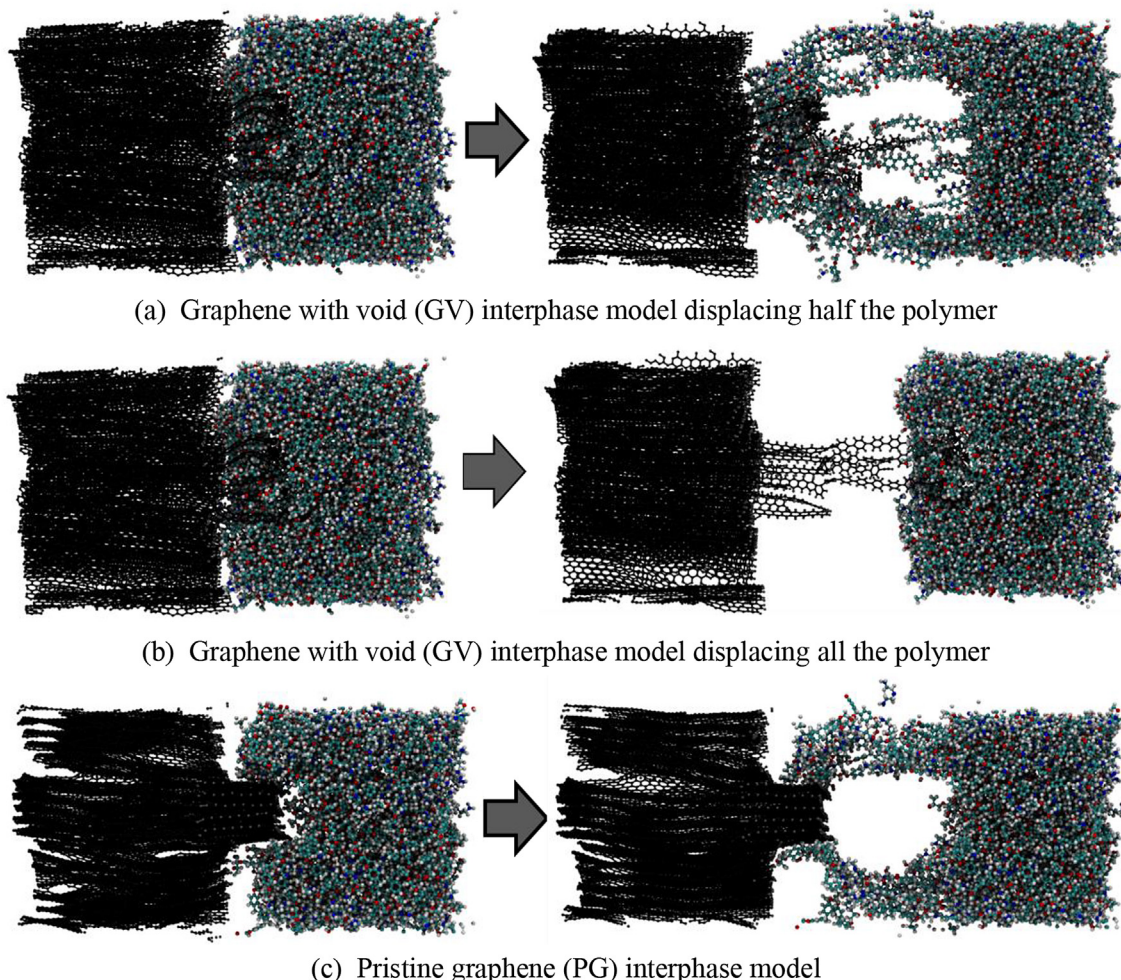
Fig. 8. Virtual test results of the equilibrated molecular interphase models showing the position of the atoms before (left) and after (right) testing.
