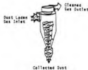
Conventional Reverse Flow Cyclone
