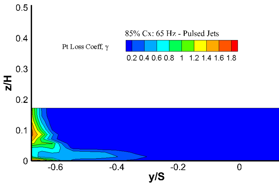
Figure 116. 65 Hz Pulsed Jets 85% Cx Total Pressure Loss Map
