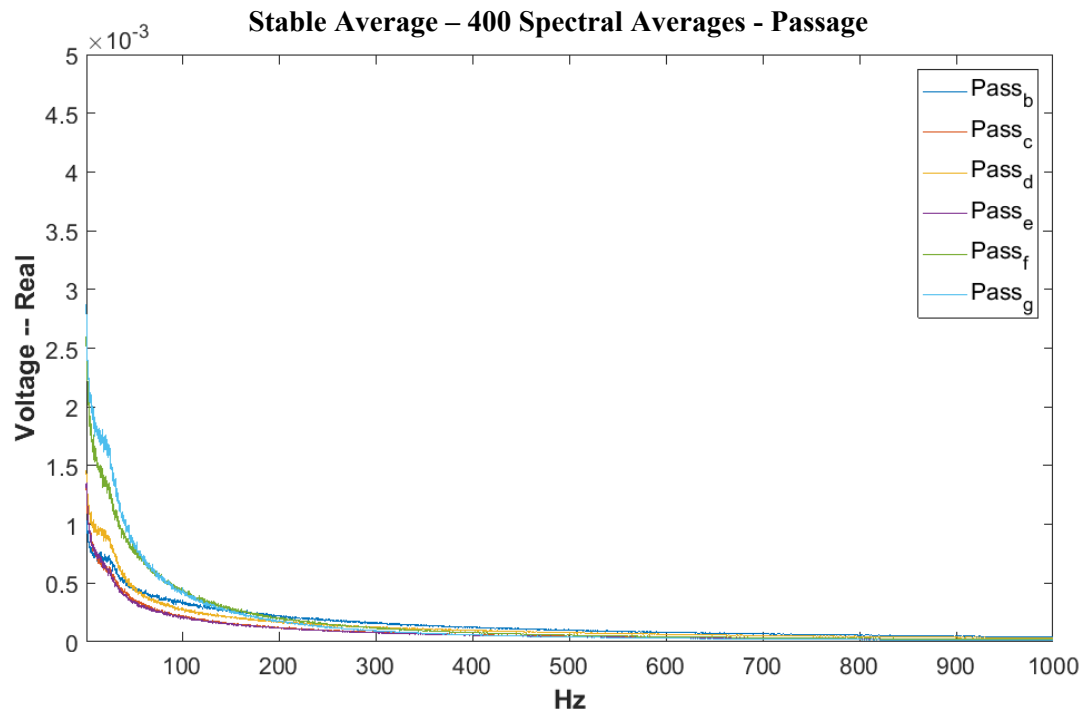
Figure 81. In-Passage Hot-film PSD, 400 Averages, 0-.005V v. 0-1000 Hz
