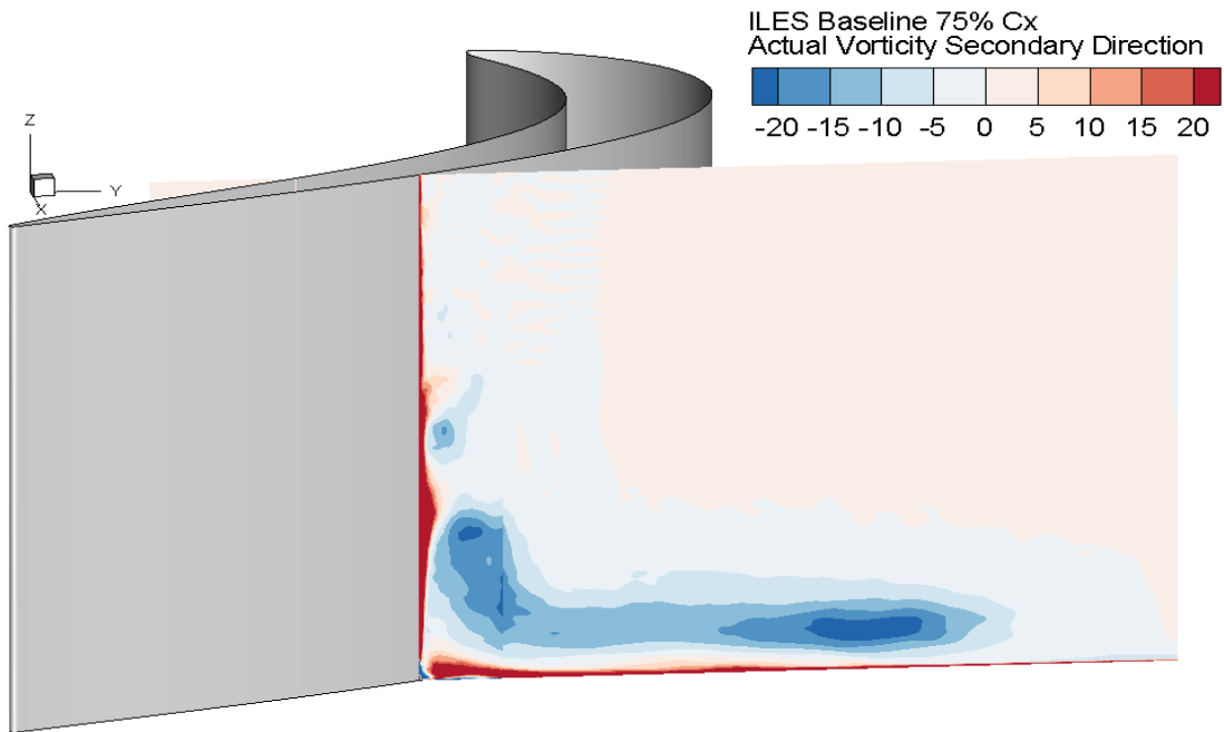
Figure 151. ILES Baseline, Actual Secondary Vorticity 75% Cx
