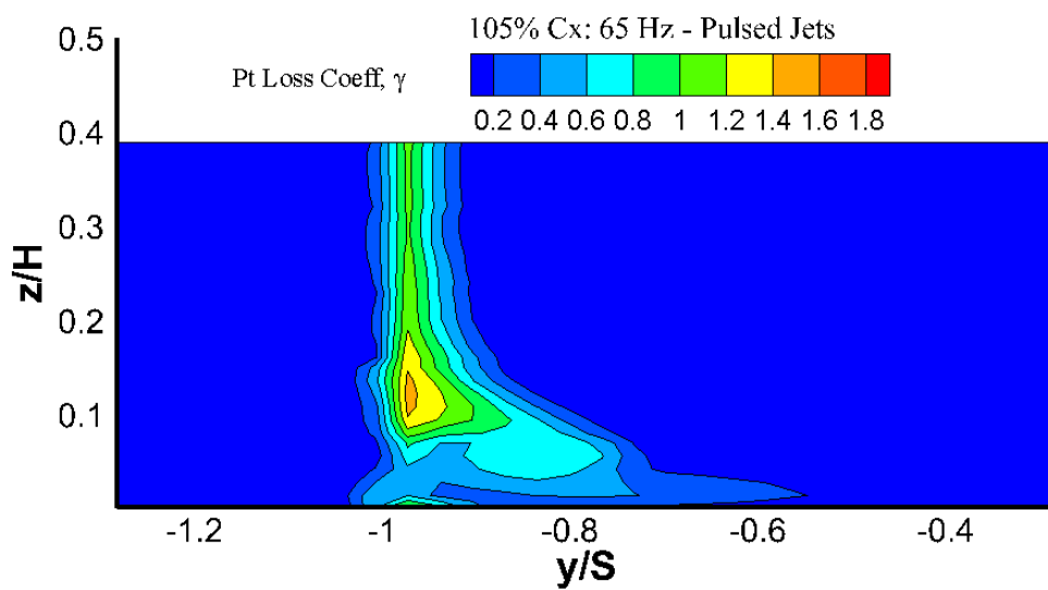
Figure 114. 65 Hz Pulsed Jets 105% C x Total Pressure Loss Map
