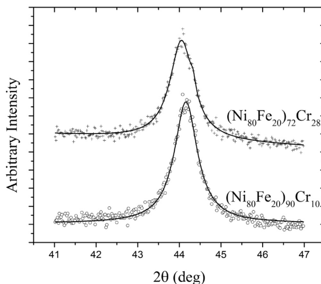
Fig. 1. Representative X-ray diffraction \theta - 2\theta scans of two (\text{Ni}_{80}\text{Fe}_{20})_{100-x}\text{Cr}_x films, showing the (\text{Ni}_{80}\text{Fe}_{20})_{100-x}\text{Cr}_x (1 1 1) peak near 44^\circ .
