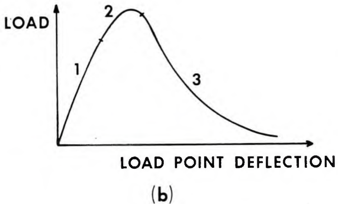
Figure 1. Three point bend test set up and load - load point deflection plot.
