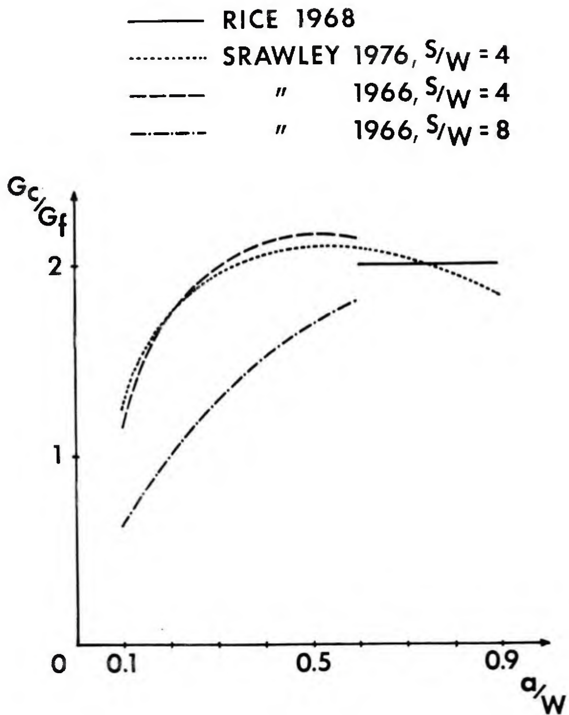
Figure 2. Ratio G_c/G_f for various crack depths.
