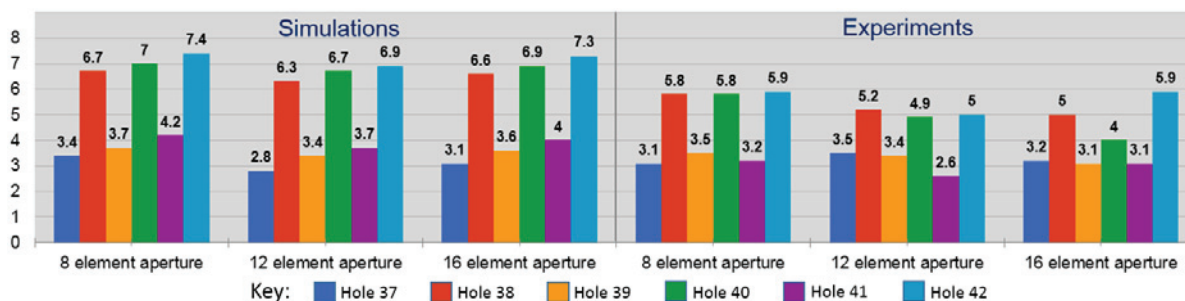
FIGURE 13. Bar charts showing hole diameters estimated from simulations (left-hand side) and experiments (right-hand side) using SAUL for the convex radius for 3 reception apertures (8, 12 and 16 elements). Actual diameters are 3 and 6 mm.
