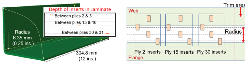
FIGURE 2. Schematic diagrams showing the CAD model for composite test specimens (left-hand image) and the location of embedded inserts at three depths in the laminate. The samples include a trim area that is available for porosity measurements.
