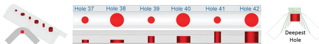
FIGURE 11. CAD model of the calibration block including the flat-bottom holes that were drilled into the convex radius (left-hand image). Top and side views of the holes are shown in the middle image. The right-hand image shows the side view of the test specimen. The green lines show the simulated beam entering the part and the beam paths in the sample.
