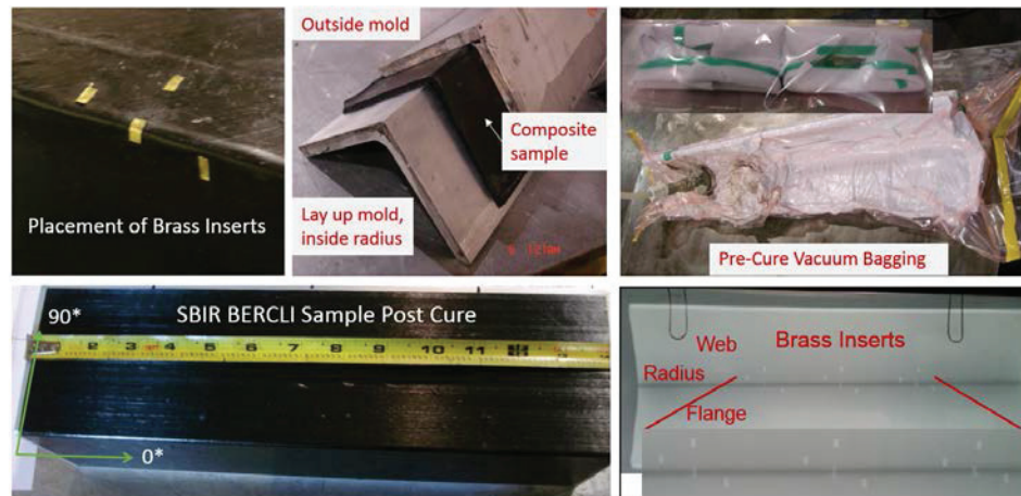
FIGURE 3. Steps in fabricating test specimens with embedded defects: placement of inserts at three depths in the laminate; vacuum bagging and autoclave cure. Radiographic imaging was performed to confirm the location of the brass defects.
