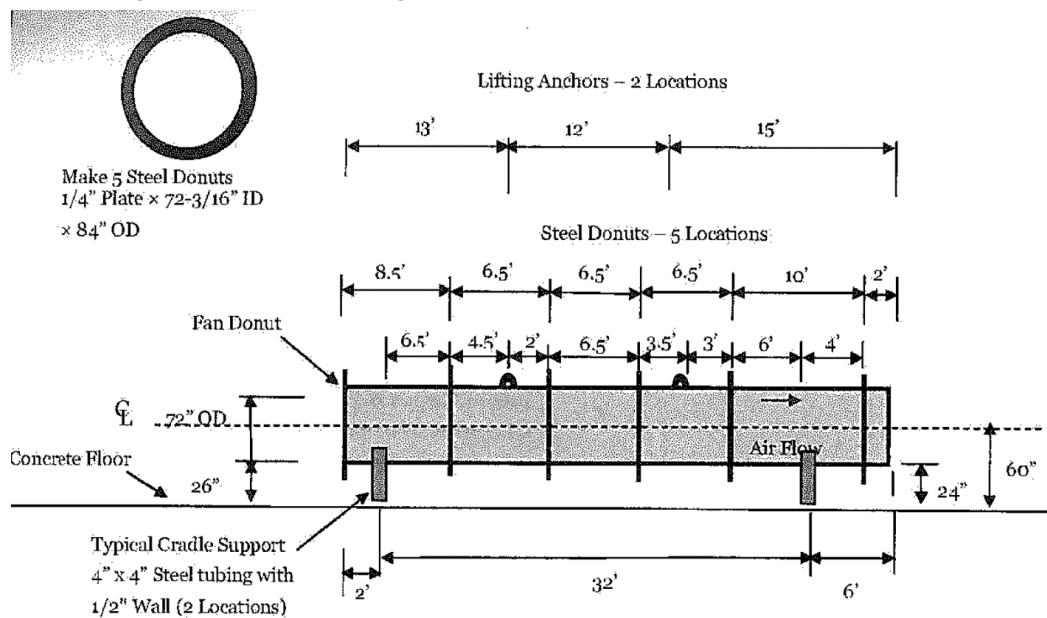
Figure A-4. Side view diagram of the GSL wind tunnel (Graham et al. 2011).
