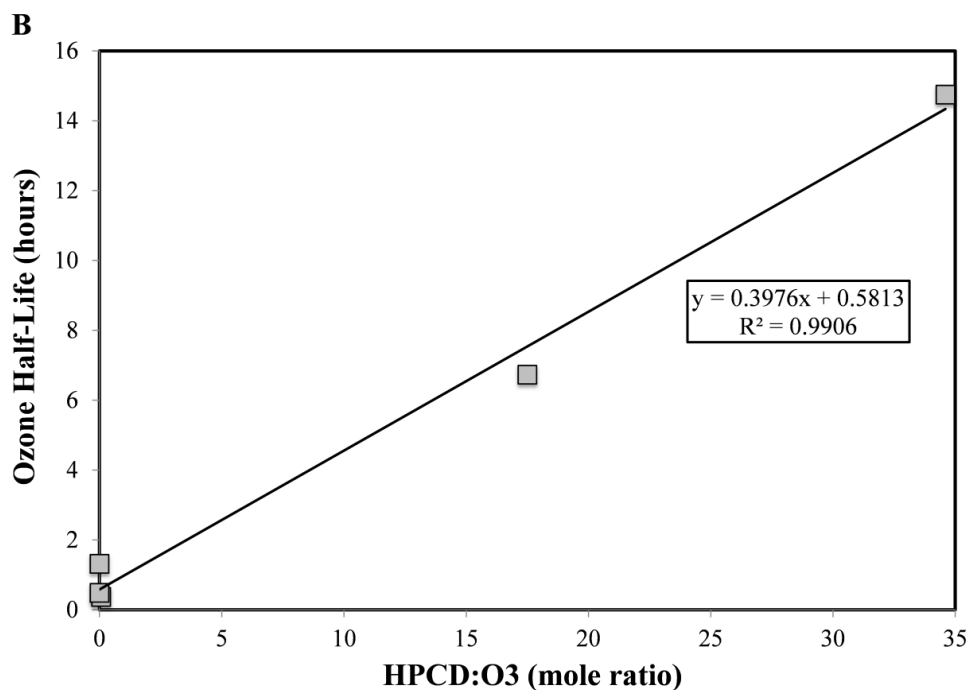
Figure 4.1.5. (A) O_3 concentration decay in groundwater solutions containing varying HP \beta CD to O_3 molar ratios. The lines are regression results assuming pseudo 1 st order (exponential) decay, and error bars represent the 95% confidence interval for triplicates. (B) O_3 half-life times plotted as a function of HP \beta CD: O_3 molar ratio, and the line presents the linear regression analysis.
