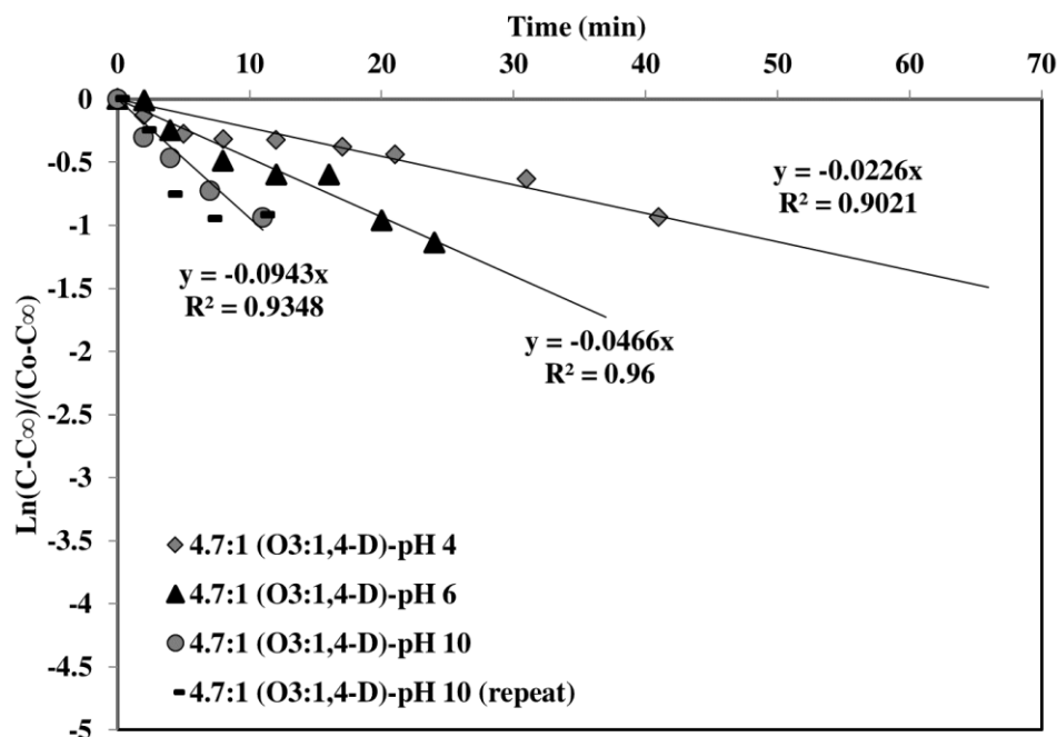
Fig. S7. Removal kinetics for 1,4-D using O_3 without HP \beta CD in multiple contaminant systems over a range of different initial pH values.
