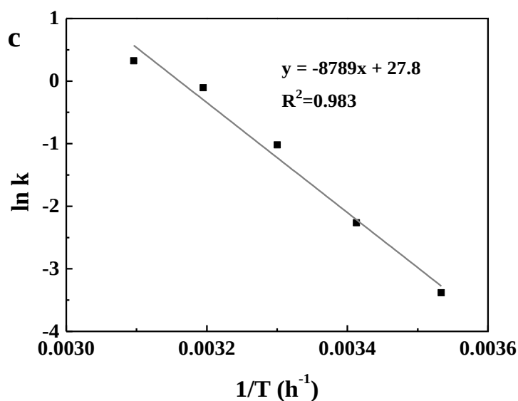
Figure 4.6.3. The activation energy for TCE degradation a) first 2 hours of reaction for the SO system; b) after 2 hours of reaction for the SO system; c) entire reaction period for the STO system.
