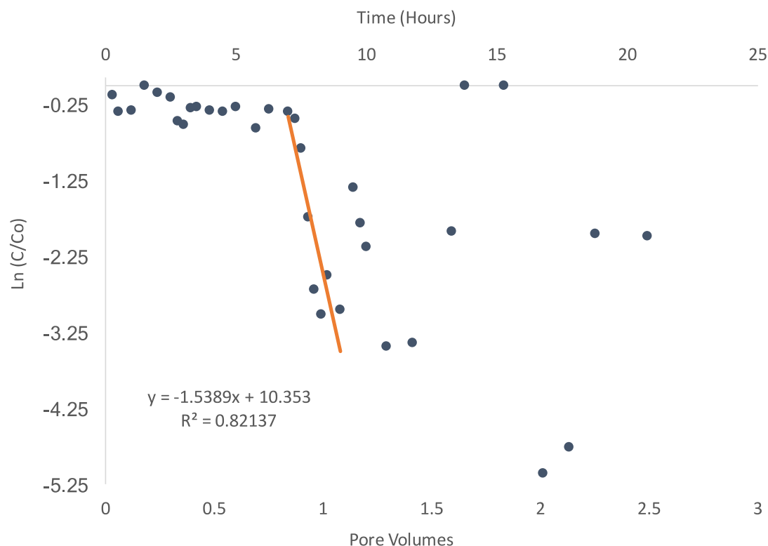
Figure 4.8.13. Results from Scenario II: \ln(C/C_0) for pseudo-first order reaction rate constant.
