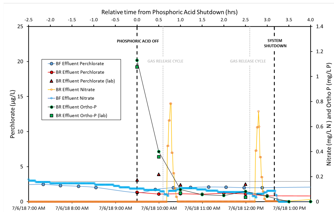
Figure 34 Phosphoric Acid Chemical Feed Failure Challenge Test
