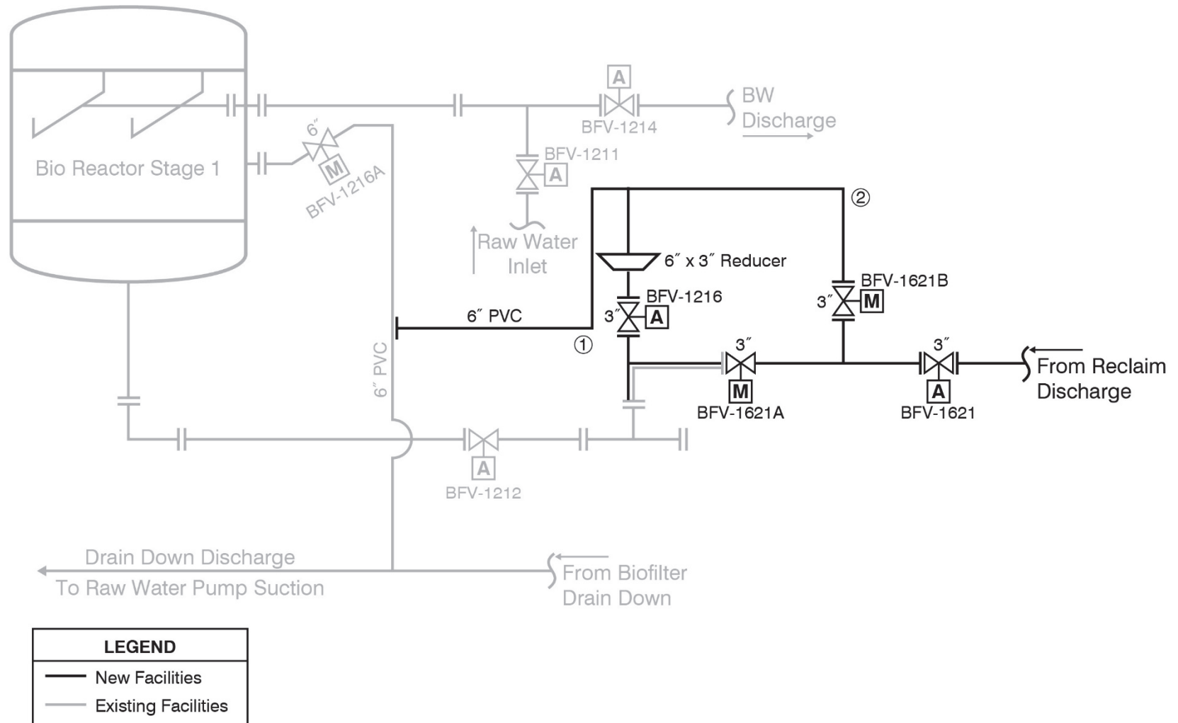
Figure C.1 Draindown Modifications
