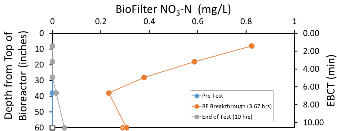
Figure 31 Biofilter Nitrate Depthwise Removal
