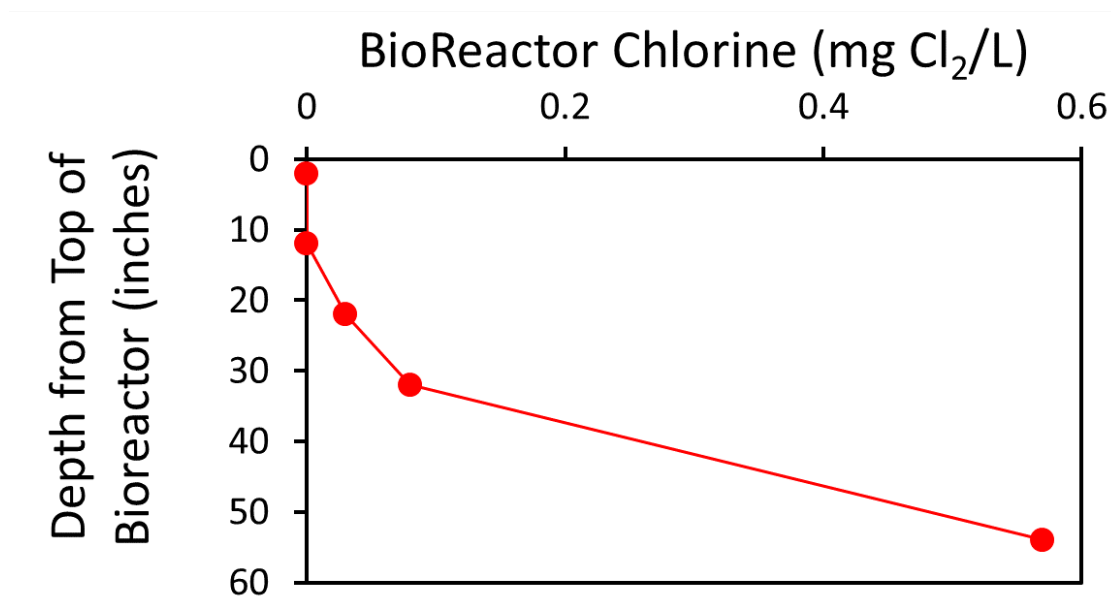
Figure 38 Chlorine Penetration into the Bioreactor
