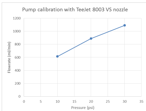
Figure 28. Calibration of Water Flow Rate Through TeeJet 8003VS Spray Nozzle
