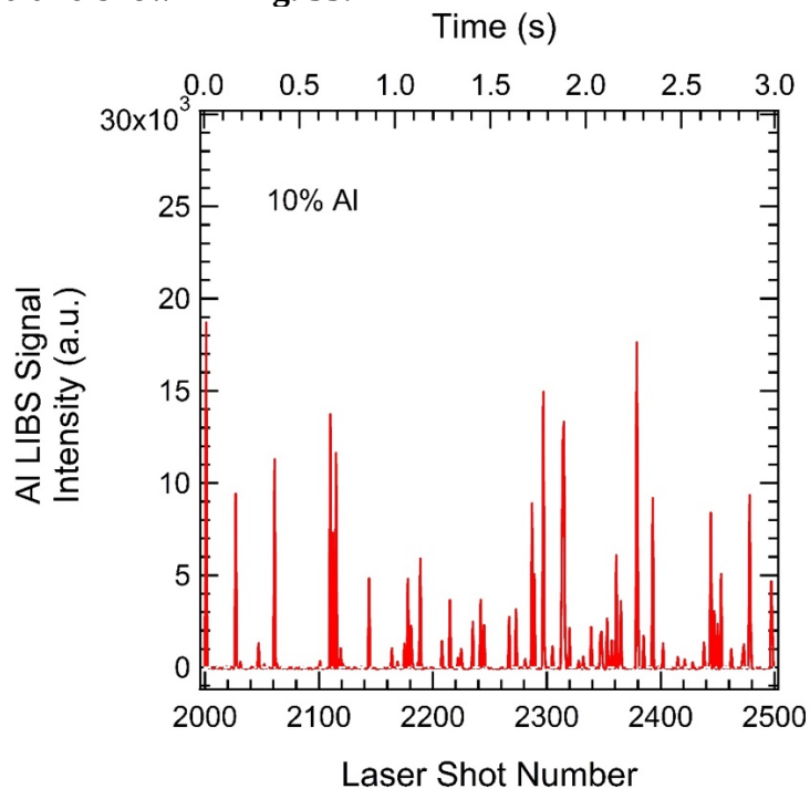
Figure 37. The data corresponding to 500 laser shots (shot range 2000 –2500) for the burn of 10% Al strand shown in Fig. 34.
