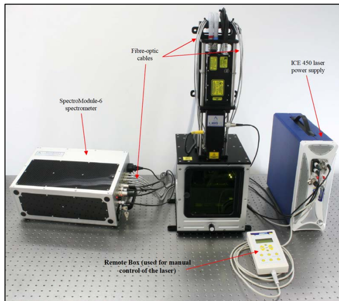
Figure 44. Compact, ruggedized, portable LIBS system acquired to our laboratory in 2018.
