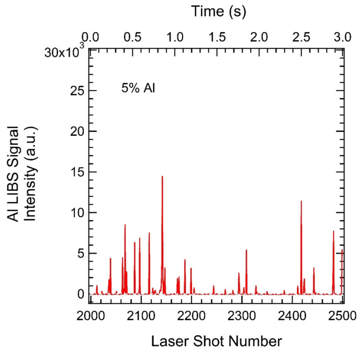
Figure 36. The data corresponding to 500 laser shots (shot range 2000 –2500) for the burn of 5% Al strand shown in Fig. 33.
