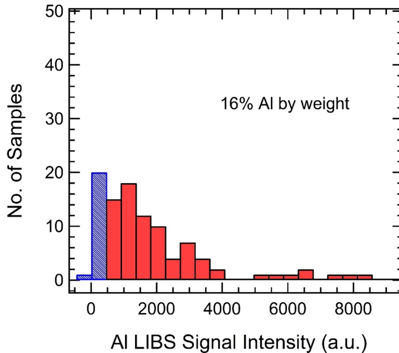
Figure 21. Histogram showing the number of samples with sufficient intensity counts shown in red and below detection limit (i.e. noise) shown in blue for 100 laser pulses during a 16% propellant strand burn.
