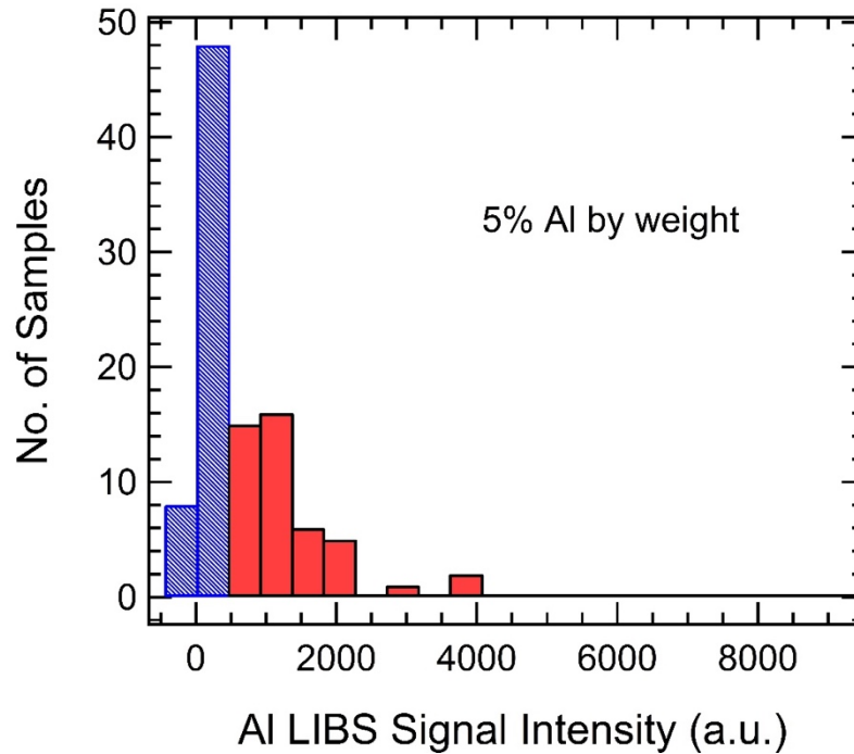
Figure 19. Histogram showing the number of samples with sufficient intensity counts shown in red and below detection limit (i.e. noise) shown in blue for 100 laser pulses during a 5% propellant strand burn.
