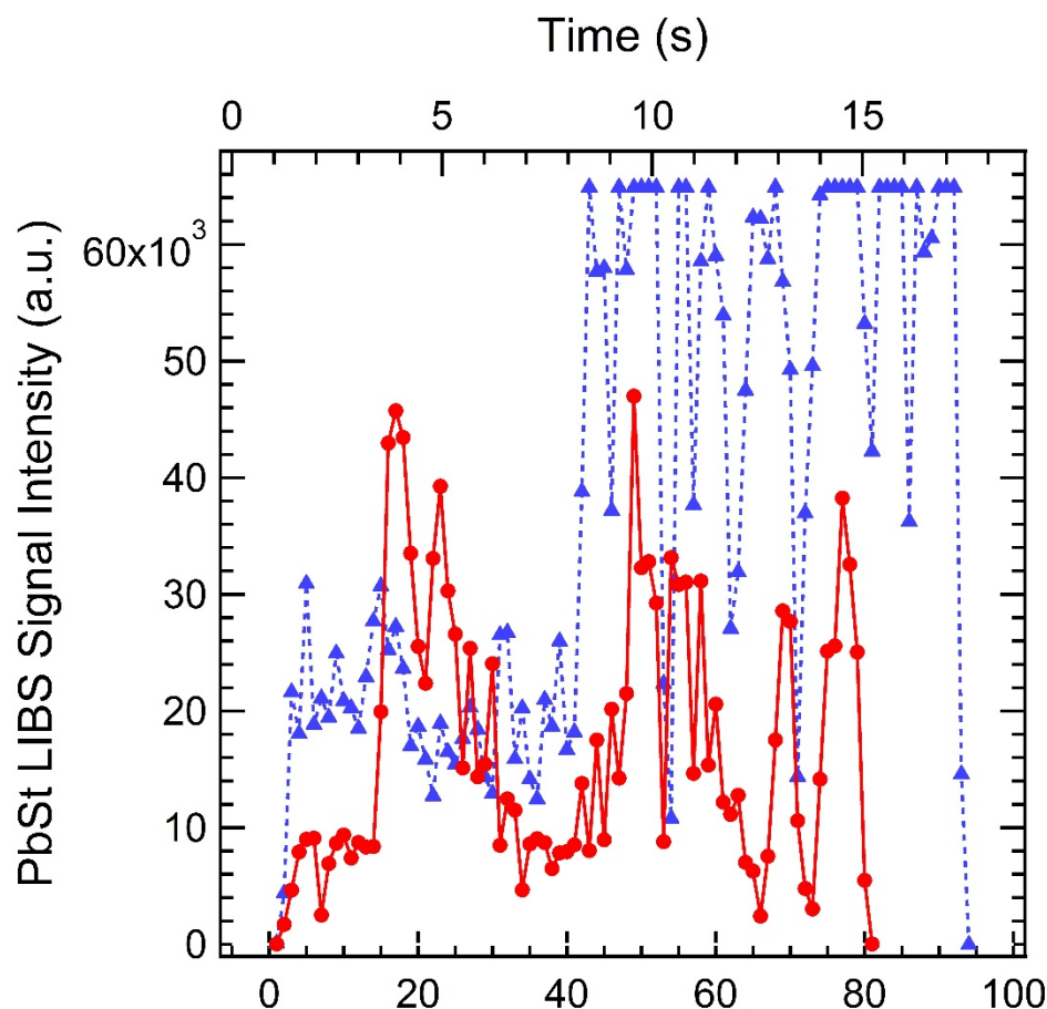
Figure 29. Time series of ns-LIBS signal of Pb extracted from two lead stearate propellant strands. The peak intensity plotted is extracted from the 405.78 nm line. Each data point represents 200 on-CCD accumulations or laser shots. The first strand, plotted in blue, had the same settings as the other burns, but it partially saturated the ICCD camera. Therefore, on the second burn, plotted in red, the gain was reduced from 10 to 6. The points are distinct frames, not a continuous signal. The lines have been added for clarification of the trend.
