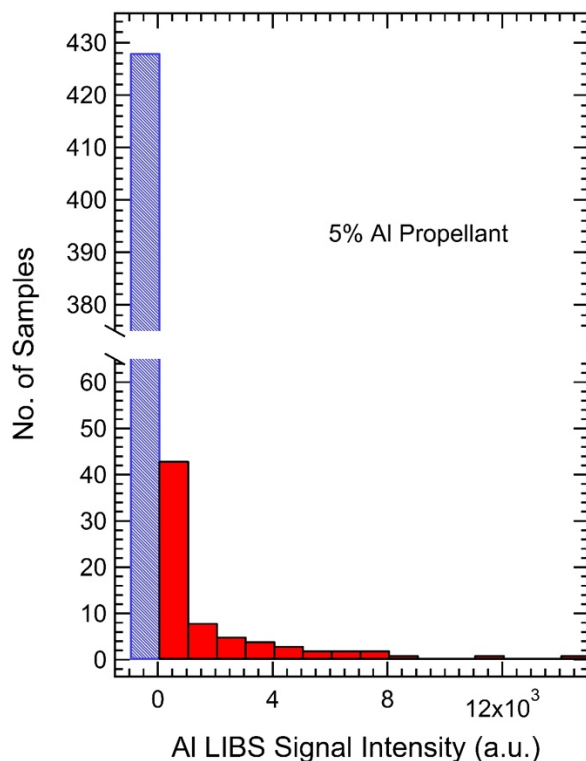
Figure 39. Histogram generated for 500 single shots with fs-LIBS of a 5% Al propellant burn. The Al LIBS signal is pulled from the peak intensity of the 396nm line.
