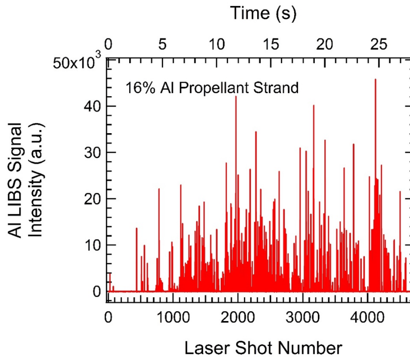
Figure 35. Single-laser-shot data of Al LIBS signal for the entire duration the burn, recorded in 16% Al propellant strand shown as a function of the laser shot number. The Al LIBS signal is extracted from the peak intensity of the 396-nm line.
