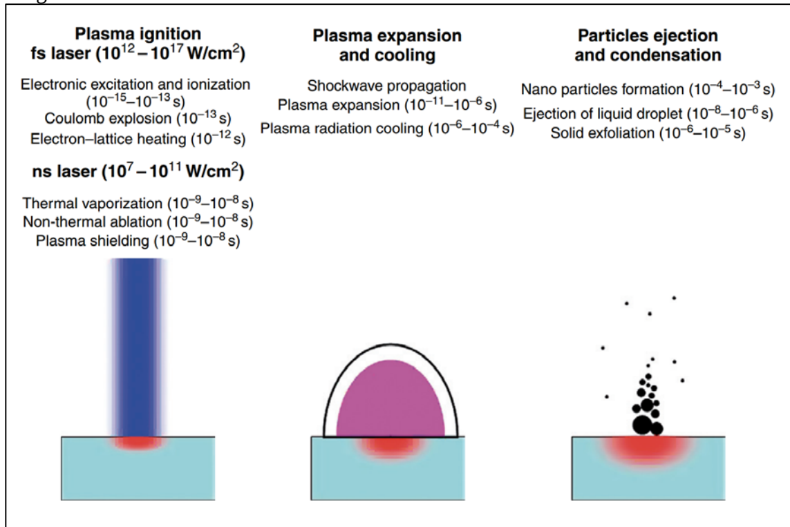
Figure 3. Schematic illustration of the main process along with respective time scales during ablation by a laser spark in a typical LIBS experiment [55]
