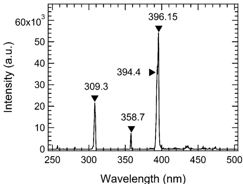
Figure 16. Aluminum emission spectrum recorded during a burning propellant strand. The peak values listed are from the NIST database. Experimental data has been red-shifted by approximately 0.5 nm to match with the NIST database.
