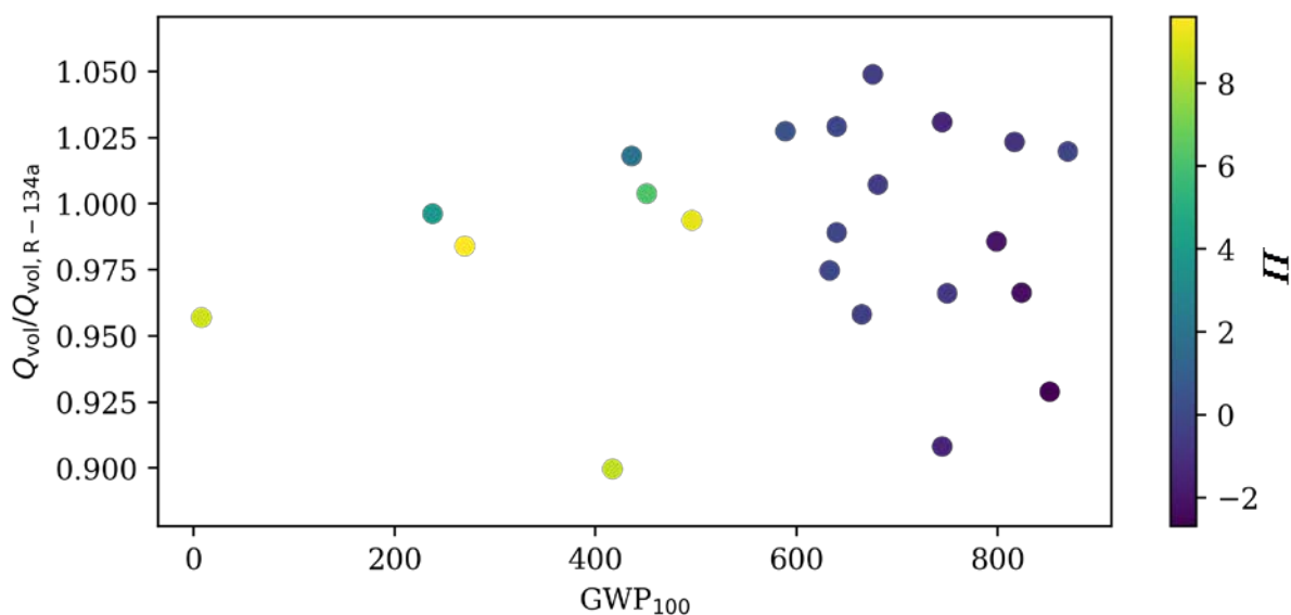
Figure 12. Q vol of the selected "best" blends (Table 2) normalized by Q vol,R-134a , plotted as a function of the GWP values; the colors indicate the estimated normalized flammability index, with the color scale on the right side of the figure.
