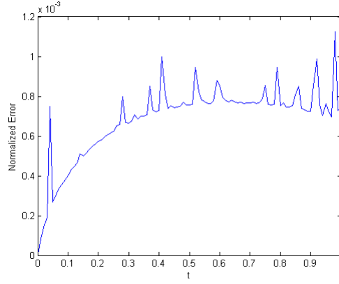
Figure 27: The RMS error as a function of t for the seventh example
