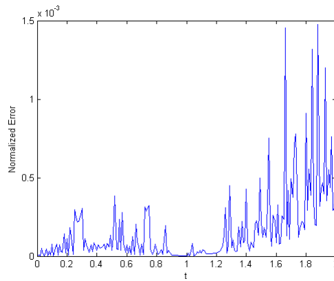
Figure 19: The RMS error as a function of t for the fifth example
