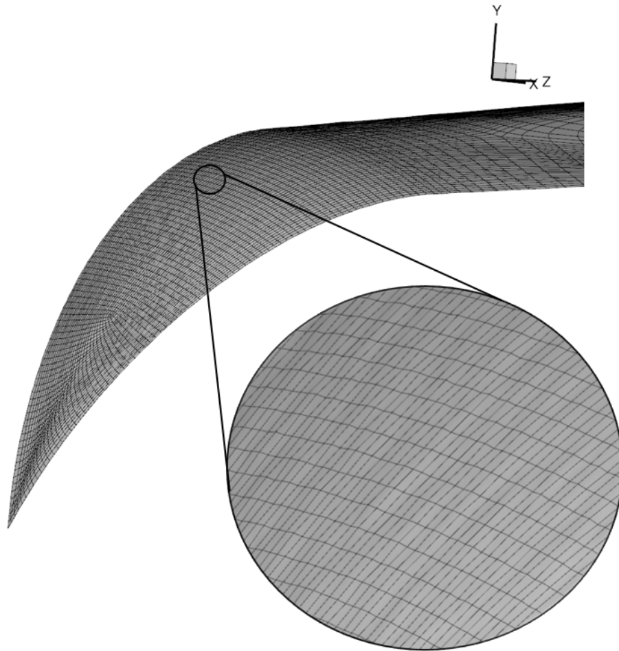
(c) Actual Surface Roughness at 15 \mu\text{m}
