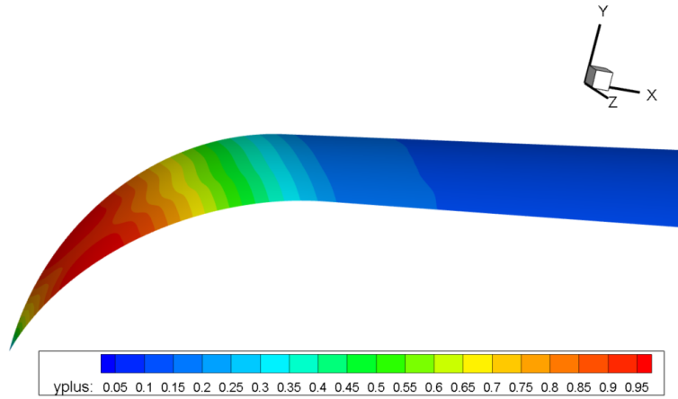
Figure 49. y^+ Contour
