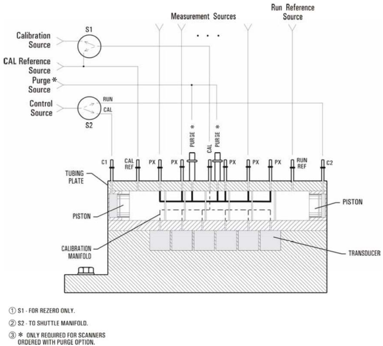
Figure II-10. Pressure scanner depiction and interfaces
