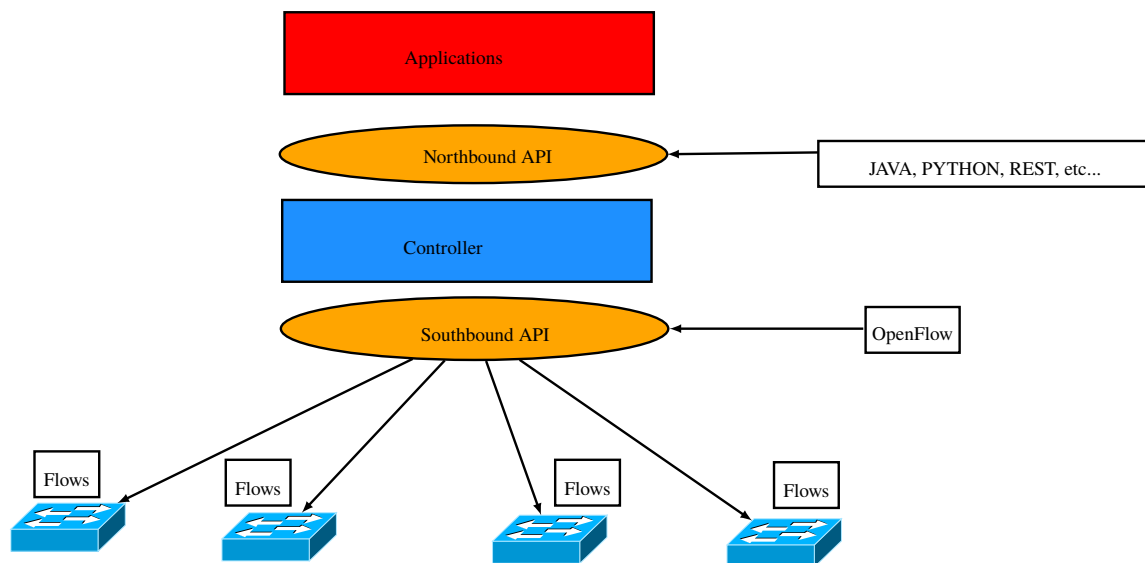
Figure 2.2. SDN Operations
