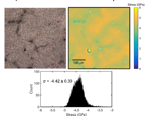
Figure 2: Optical image and extracted stress profile of Single crystal Rene N5 TBC alloy materials. Lower panel: Stress distribution.
