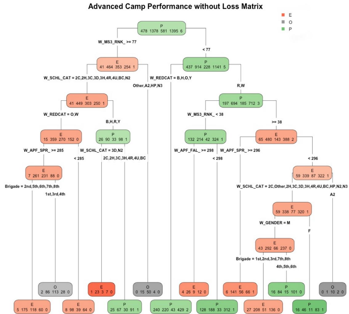
Figure 23. Classification Tree for Advanced Camp Performance without Loss Matrix
