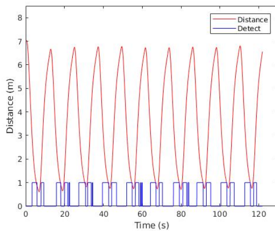
Figure 40. LRC 0.5 m test
