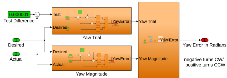
Figure 22. Yaw direction and magnitude selector
