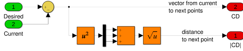
Figure 25. Simulink code that calculates the vector \overline{CD}
