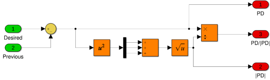
Figure 26. Simulink Code that calculates the vector \overline{PD}
