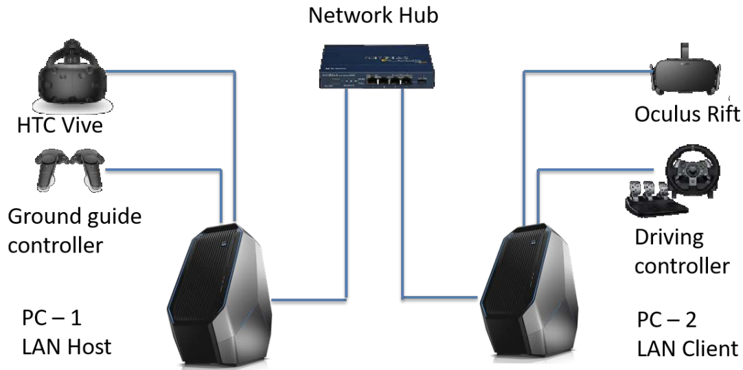
Figure 9. System architecture
