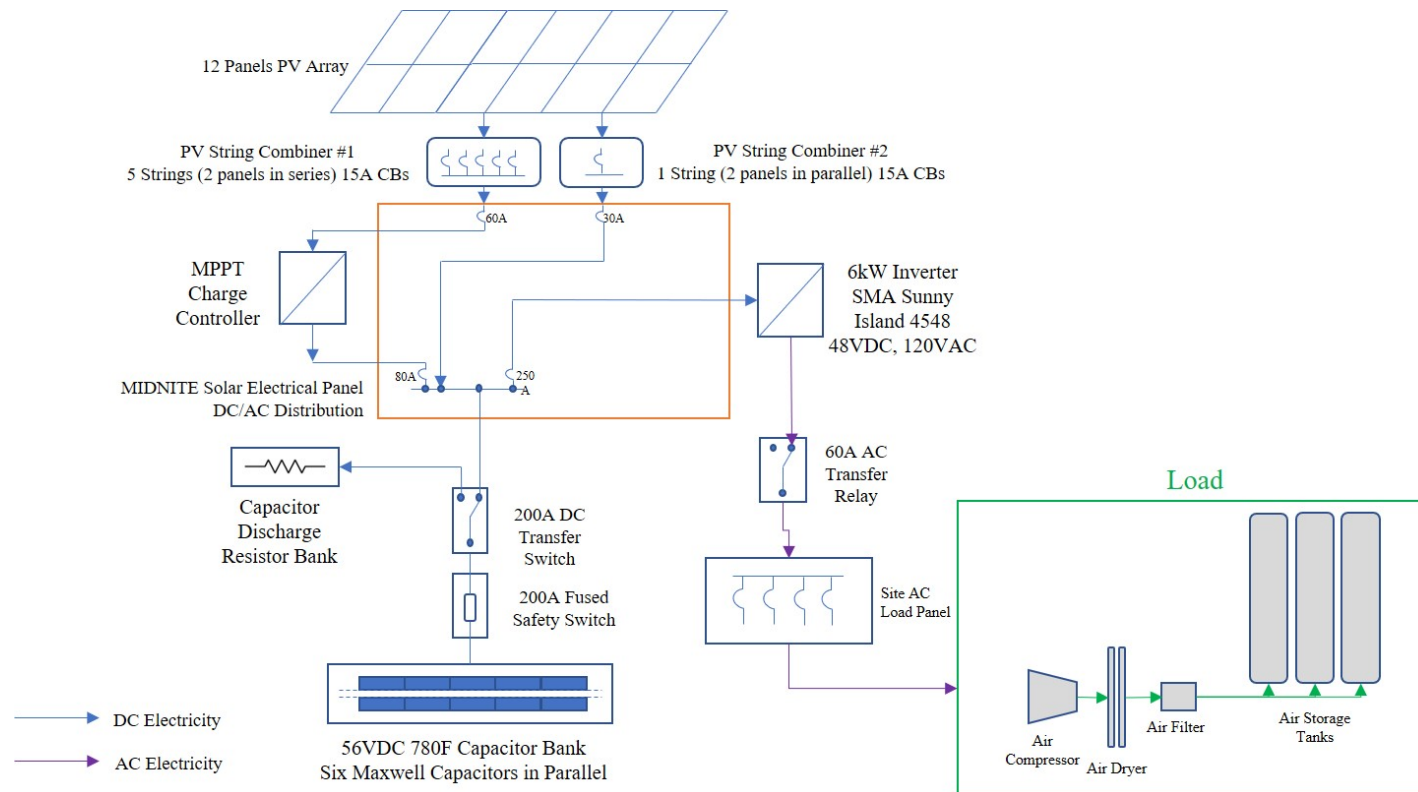
Figure 17. System Architecture of SS-CAES Compression Phase.
