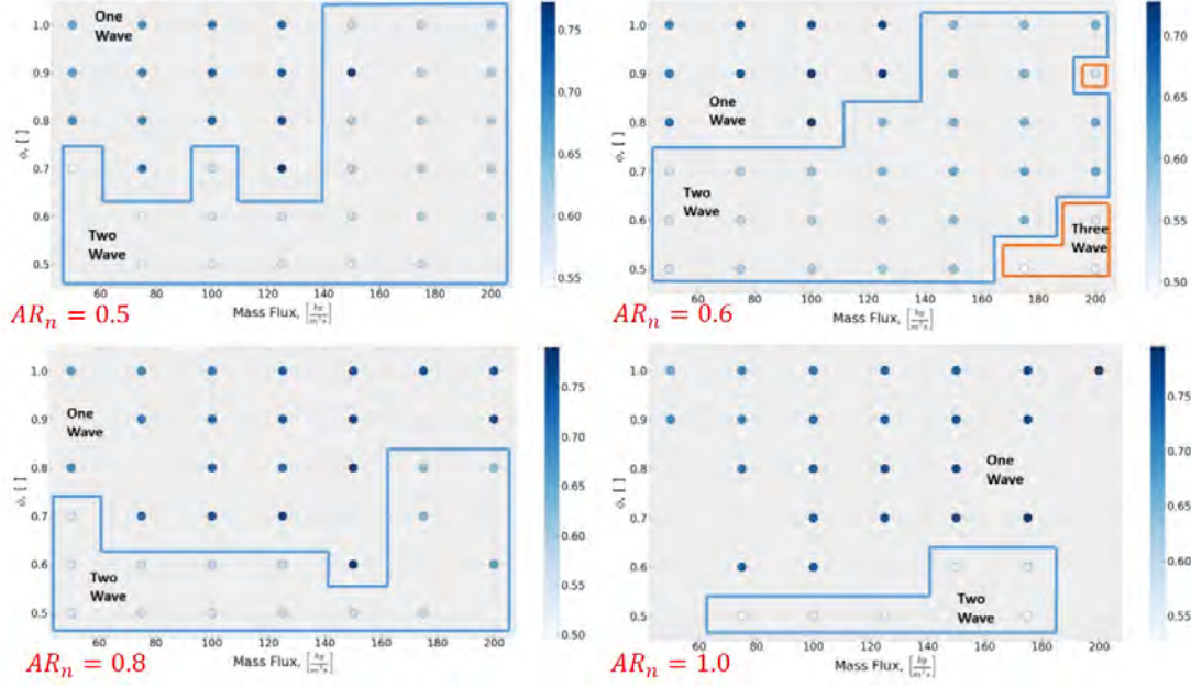
Figure 23. RRDE operability maps at Channel Height = 4.5mm, AR_t = 0.2 . Colored by v_D/v_{D,CJ} . Compiled from Huff [41], with AR_n labels added for clarity.
