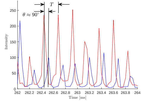
(d) Intensity traces at the the ITP locations from Test 1 for N_D = 2 operation.
