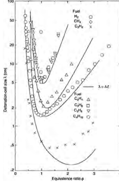
Figure 14. \lambda increases monotonically away from \phi = 1 for a variety of common detonation fuels. From Knystautas et al. [24].
