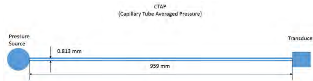
Figure 33. Schematic sketch of a notional CTAP measurement device from Stevens et al. [50]
