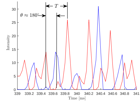
(f) Intensity traces at the the ITP locations from Test 6 for three node acoustic operation.
