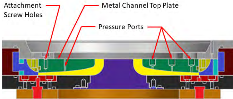
(a) Baseline metal channel top plate
