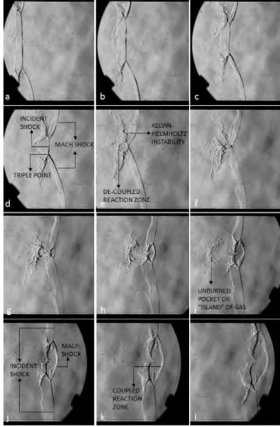
Figure 9. Detonation of a CH_4 + 2O_2 mixture at an initial pressure of 3.5kPa , with images at 11ms intervals. From Maxwell et al. [20].
