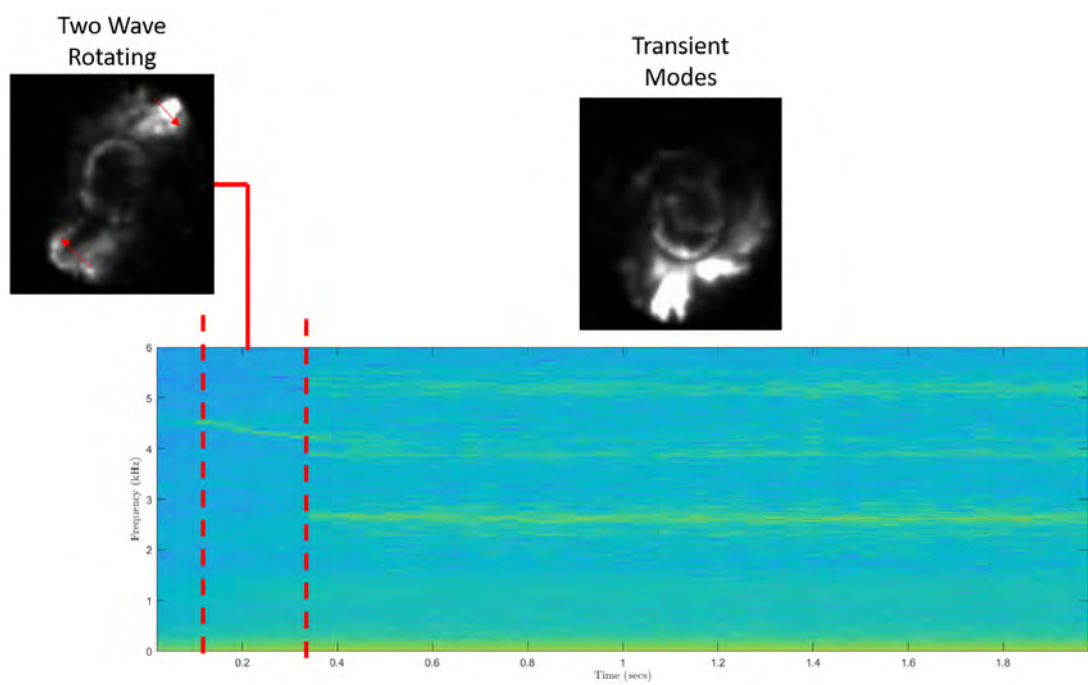
Figure 121. Test 17 Mode Persistence
