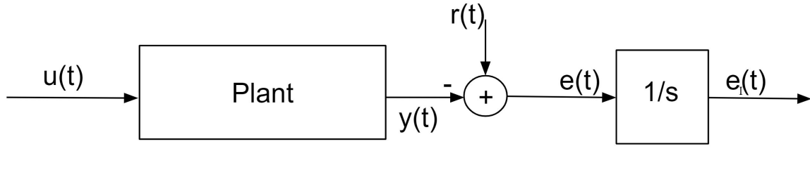
Figure 9. LQR Integral Control Augmentation
