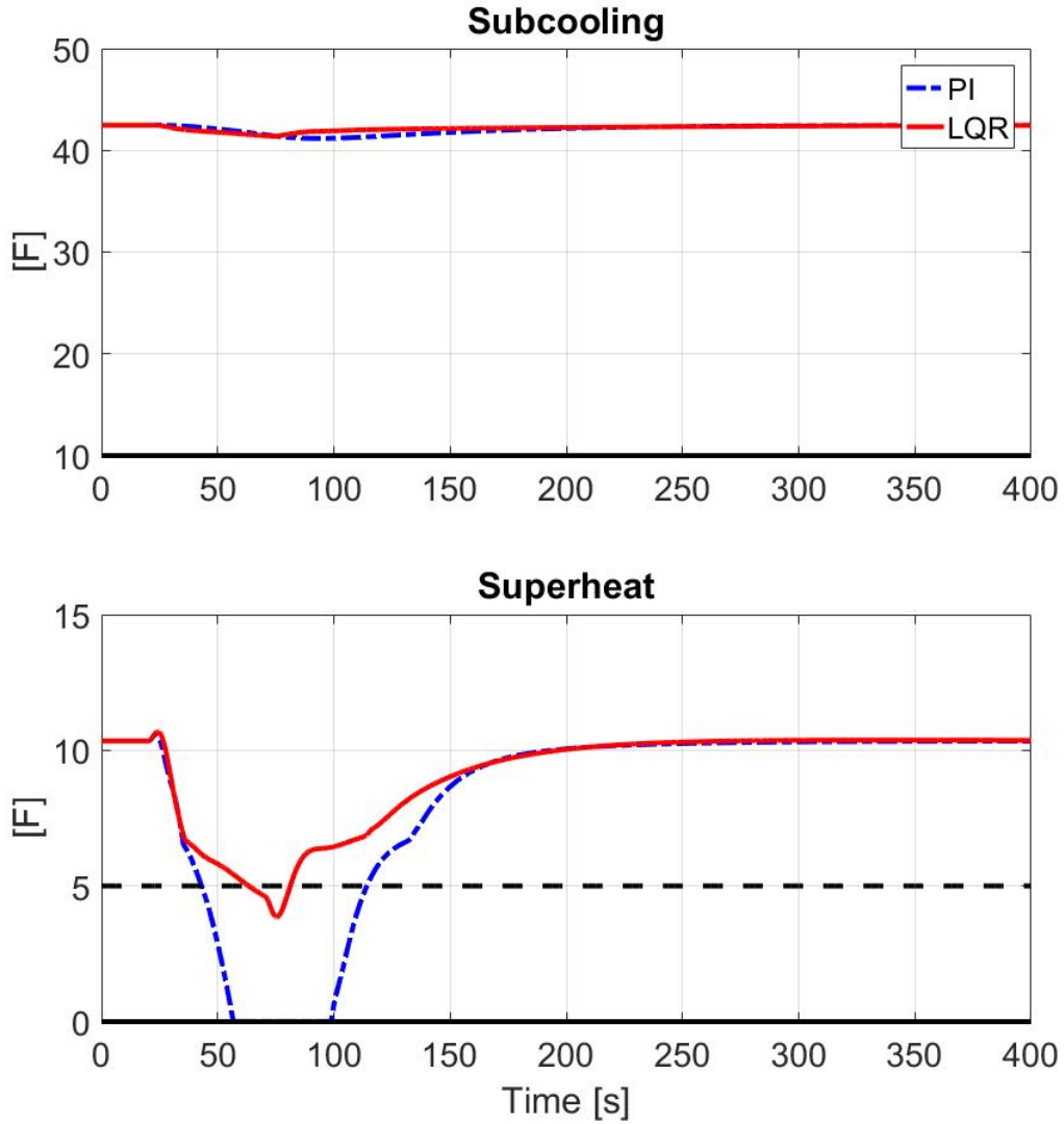
Figure 13. Simple VCS: Uncontrolled Outputs
