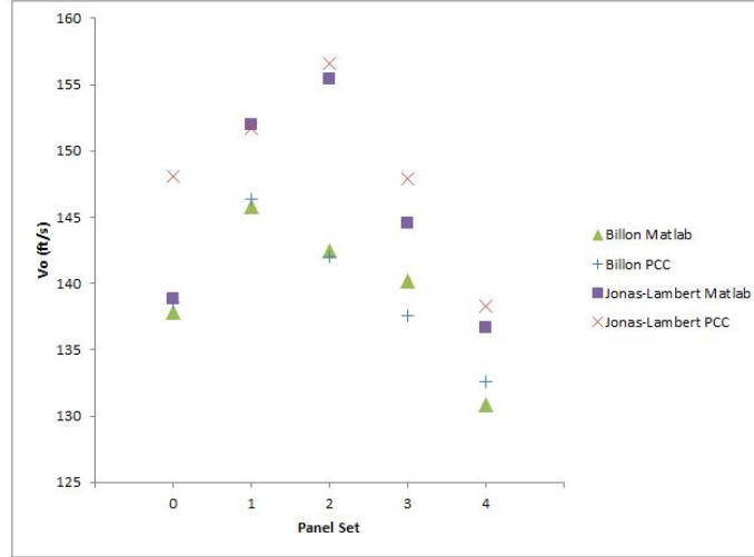
Figure 51. Comparison between the Jonas-Lambert method and Bilon method estimates of the limit velocity for each panel configuration using both the camera software (PCC) velocities and the MATLAB digital image correlation (DIC) values
