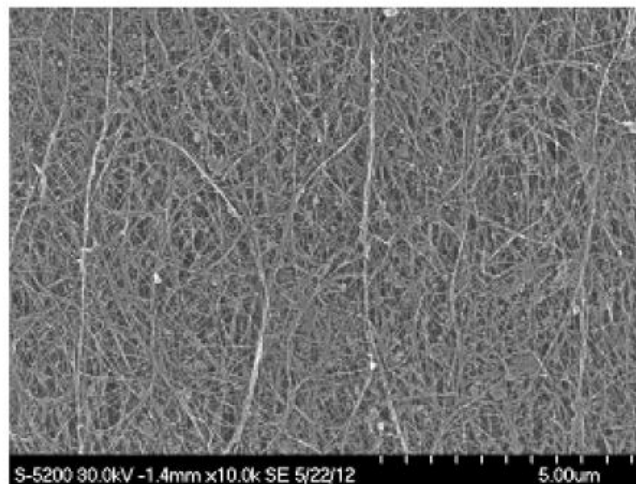
Figure 5. High resolution SEM image of CNT sheet surface, 10 \mu\text{m} by 10 \mu\text{m} area. Used with permission. [29]
