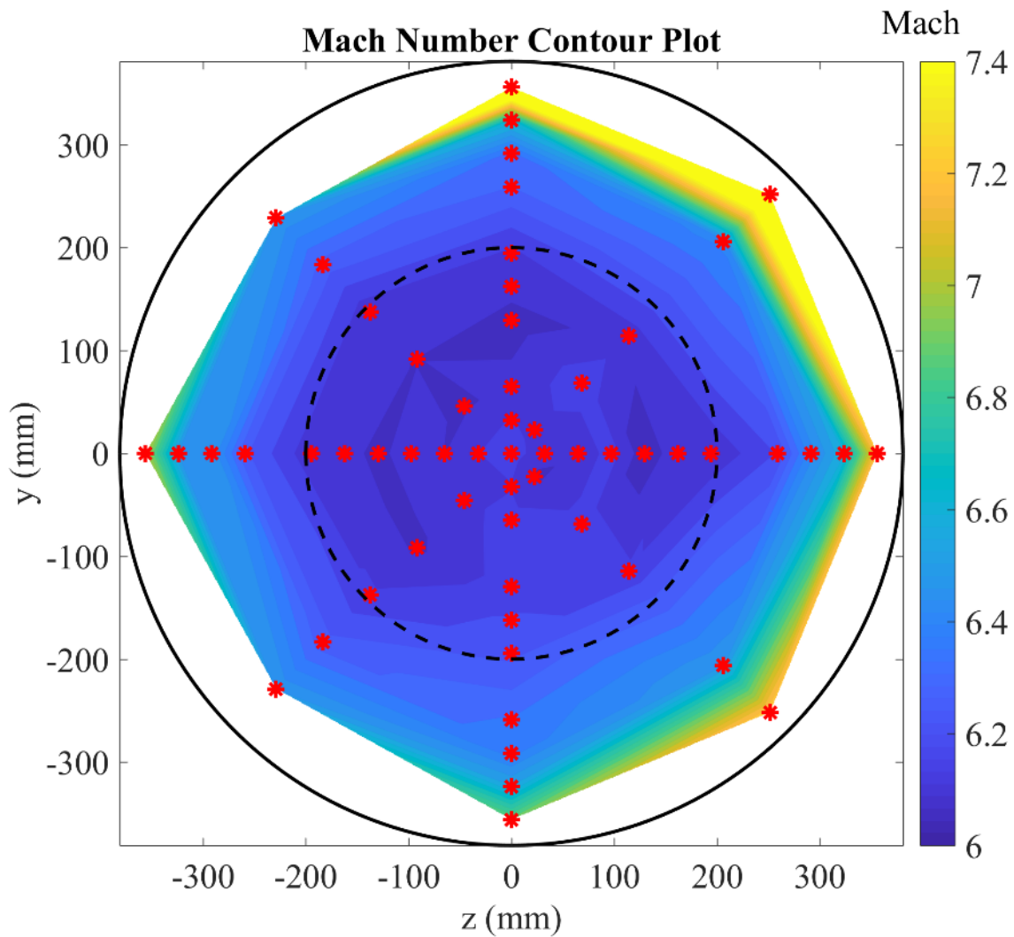
Figure 19. Mach Number Contour Plot (x=815mm)
