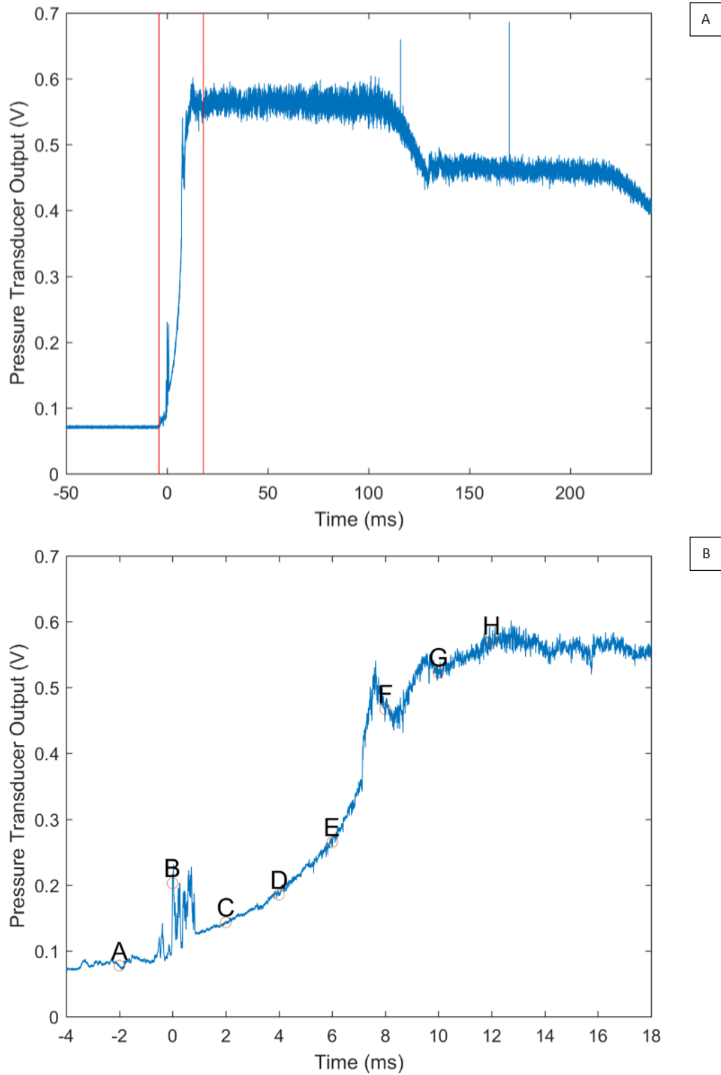
Figure 22. Pressure Trace
