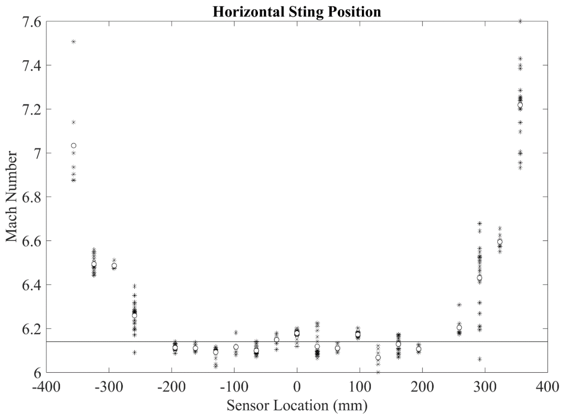
Figure 20. Mach Number Measurements Across the Horizontal Sting Position (x=815mm)
