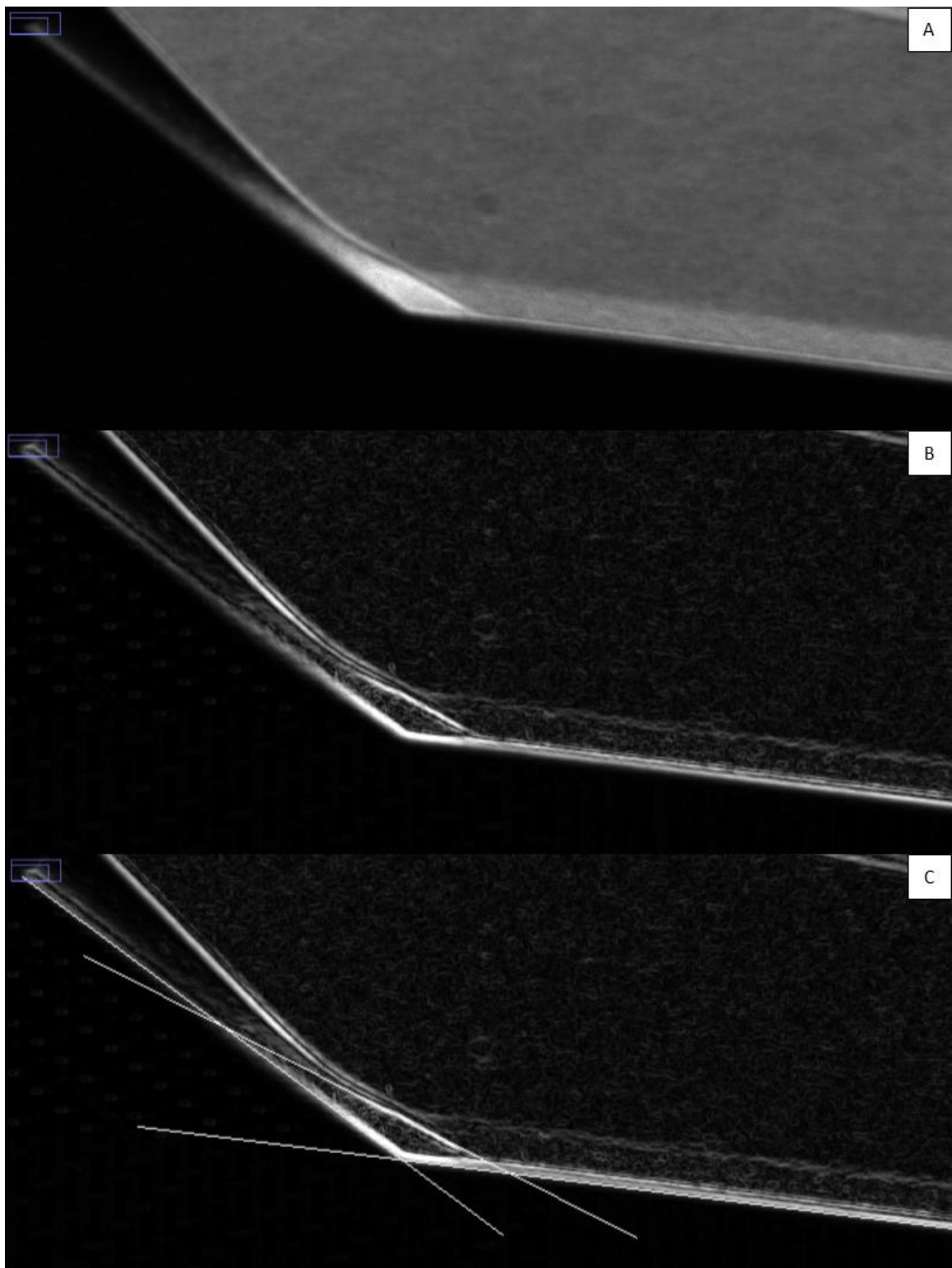
Figure 42. Recirculation Region Measurement Process (A): Standard Deviation Image (B): Post 'Find Edges' (C): Projecting Regions of interest
