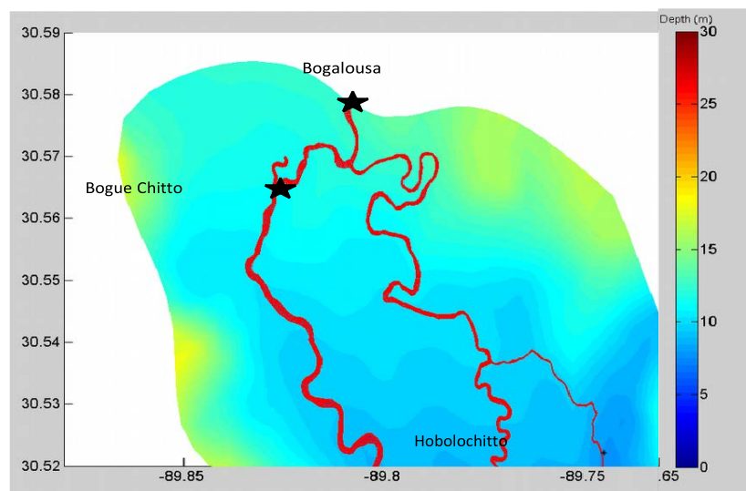
Figure 15 – Upstream bathymetry of the LPRB model near the West and East Pearl River confluence. Active discharge locations (stars), Bogalouza, LA (BXAL1) and Bogue Chitto, LA (BSHL1).
