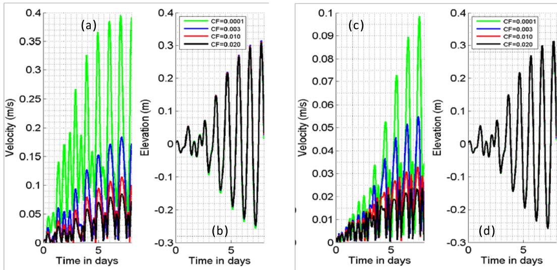
Figure 7 – Modeled currents and water levels using different friction coefficients for (a) Velocity (current) and (b) Elevation (water level) on the West Pearl; (c) Velocity and (d) Elevation on the Middle Pearl.
