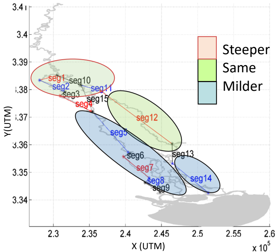
Figure 8 – The variation of topographic slope in the West Pearl and East Pearl river segments compared to the constant representative slope ( -3.3832 \times 10^{-4} ) applied over the entire Pearl River channel model.
