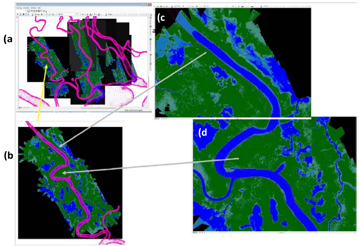
Figure 4 – (a)&(b) West Pearl River channel mesh developed from earlier satellite based remote sensing imagery compared to (c)&(d) a recent (December 2014, Mississippi State University) land/water mask derived from UAS imagery of the West Pearl River and its surrounding floodplain in Louisiana.
