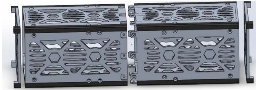
Figure 3.1. Roberts' Male/Female Interface Design [11]
