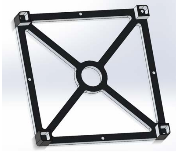
Figure 6.2. Endplate Model
