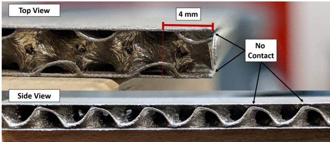
Figure 5.18. Gyroid 2 Beam
