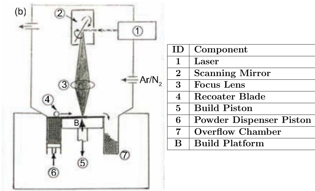
Figure 2.8. LPBF system schematics [35, 15, 39]
