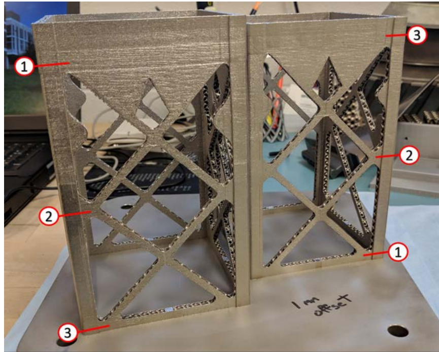
Figure 6.10. Width Measurement Locations
