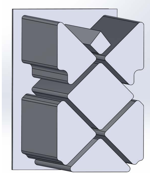
Figure 6.6. Truss Cutout Extrusion
