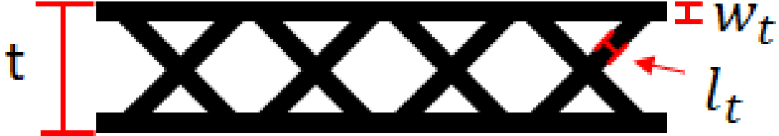
Figure 5.4. Lattice Wall Variable Descriptions
