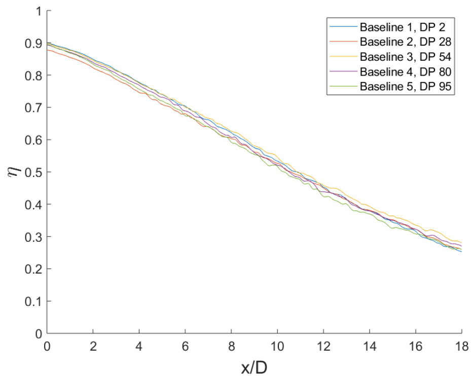
Figure 38: Centerline \eta_M for all baselines using the weighted average interpolation.
