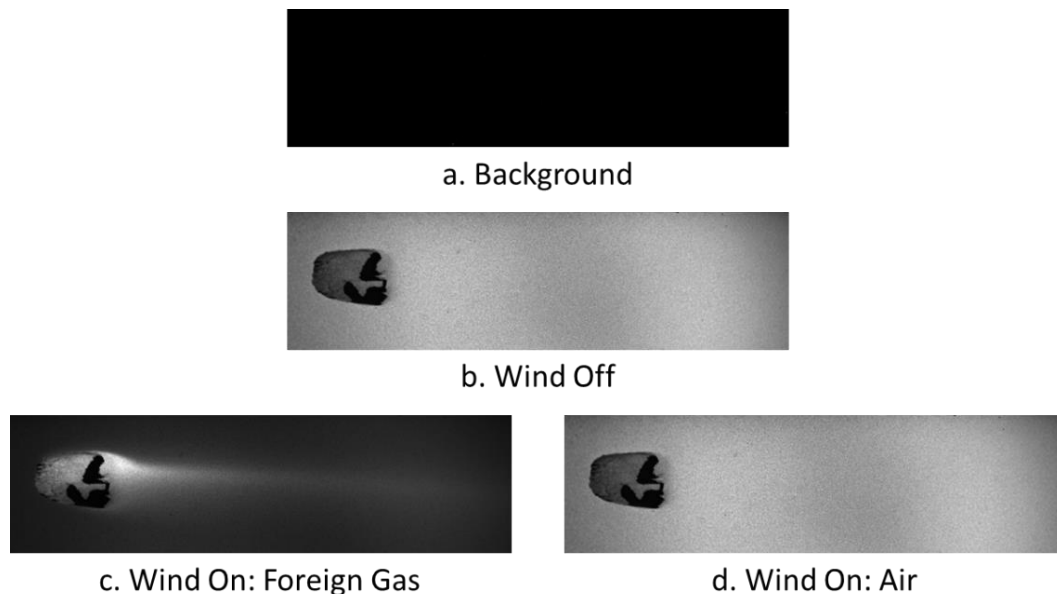
Figure 32: CCD camera images for pressure sensitive probe: reference images a) and b), test images with coolant c) and d).
