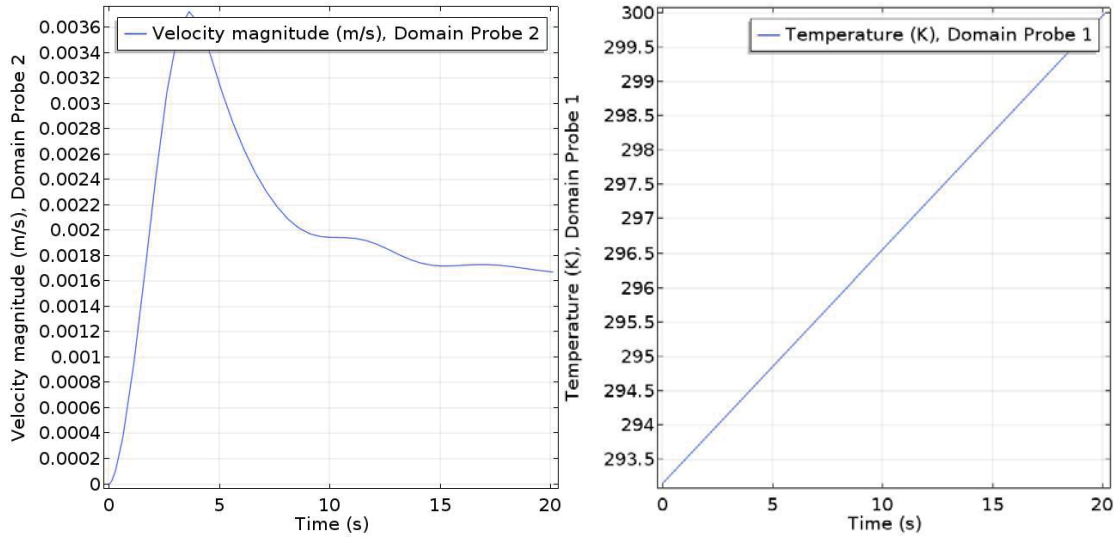
Figure 20: Maximum velocity magnitude and average temperature in f(x) heated drop P2+P1 discretization and no stabilization
