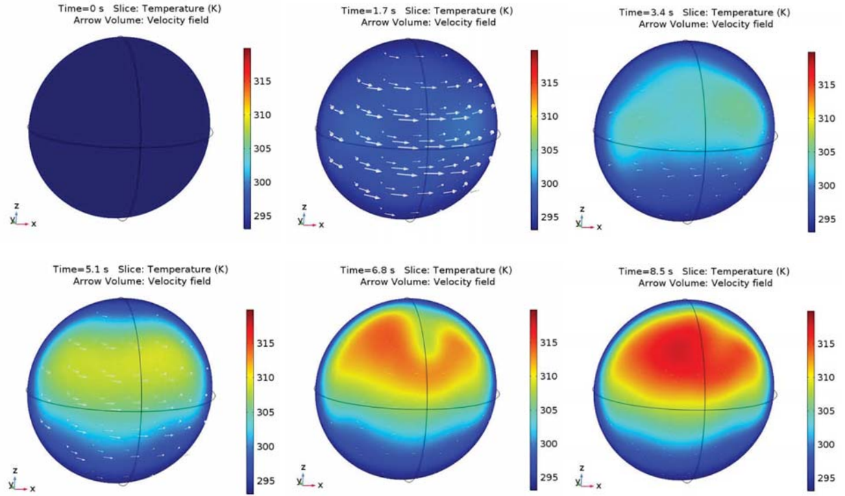
Figure 28: Temperature profiles and velocity fields for laser-heated drop with convection and body forcing function
