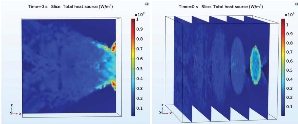
Figure 23: Laser heat field from sphere ray tracing applied to cube shaped domain
