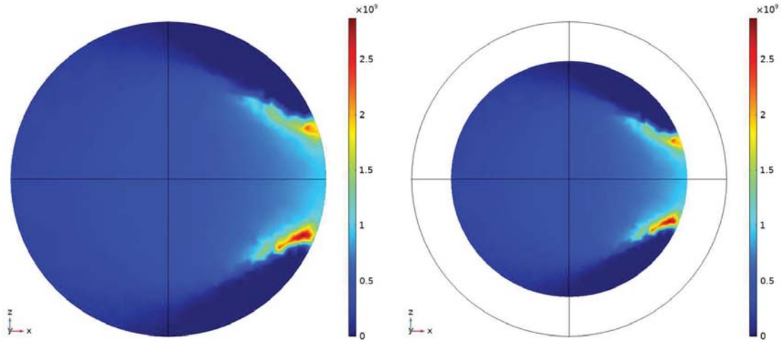
Figure 32: Heat field in shrinking drop at t=5 seconds (left) and t=25 seconds (right)
