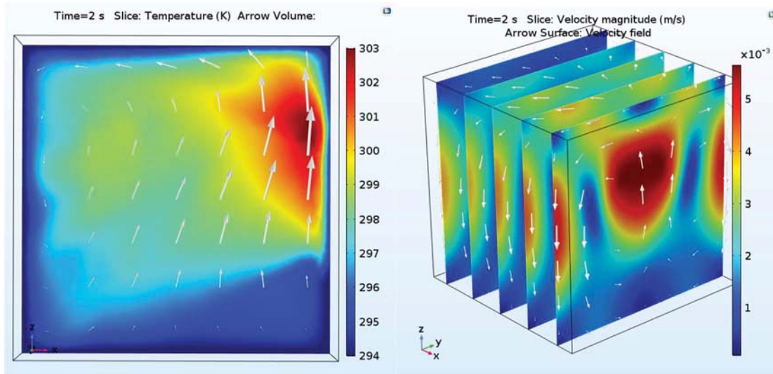
Figure 24: Temperature (left) and velocity (right) profiles from a convected and heated water cube
