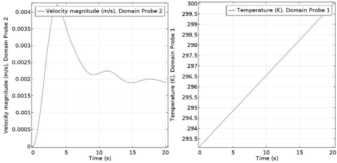
Figure 19: Maximum velocity magnitde and average temperature in f(x) heated drop
