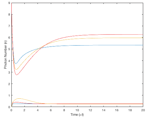
FIG. 20: Time propagation of the semiclassical equations for \Delta\omega/\kappa = 0 , g/\kappa = 10 , \gamma/\kappa = 16 , \mathcal{E}/\kappa = 4.05 , J/\kappa = 0.2 . Symmetry-preserving (blue) and symmetry-breaking solutions for one high photon number cavity (red) and two high photon number cavities (yellow).
