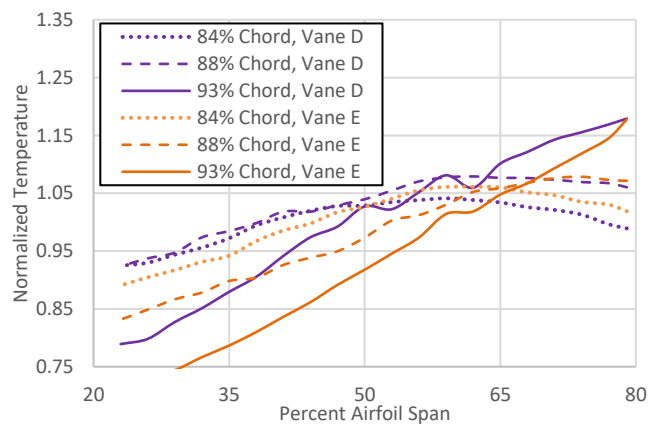
Figure 84: Vane D and E radial temperature at three axial chord locations for Case 2
