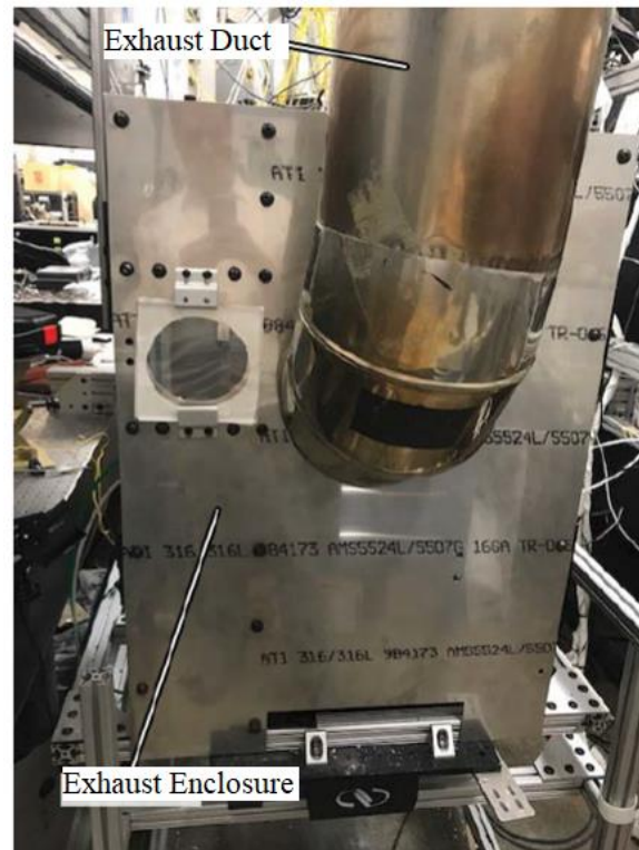
Figure 46: COAL lab initial exhaust enclosure and optical access point [33]
