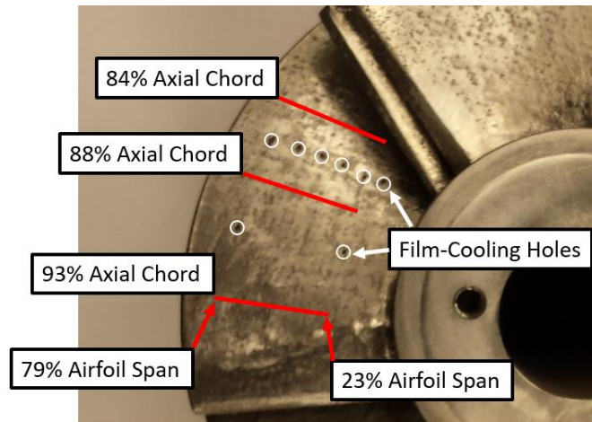
Figure 63: Axial locations of radial temperature readings
