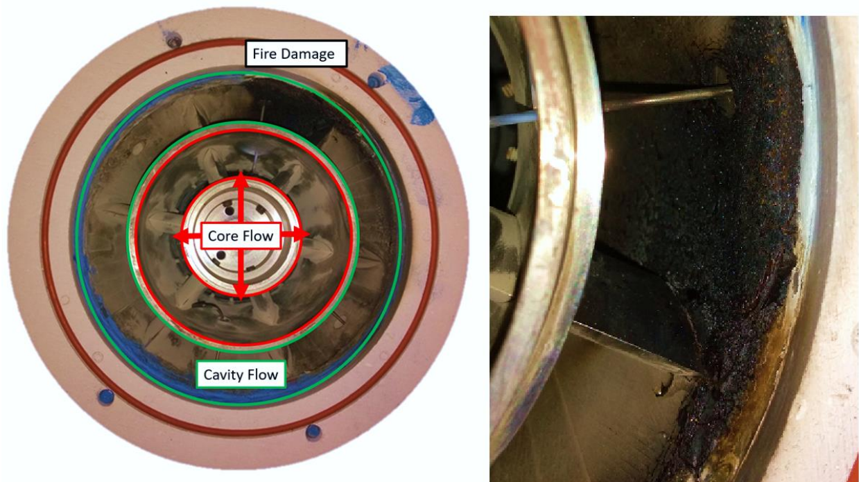
Figure 52: Fire damage from ignition jet viewed from the downstream side of the diffuser
