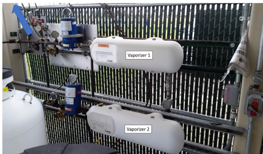
Figure 51: COAL lab fuel vaporizers [33]
