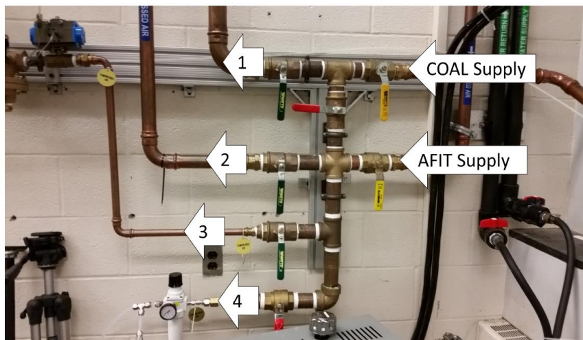
Figure 48: COAL lab initial air distribution system [33]
