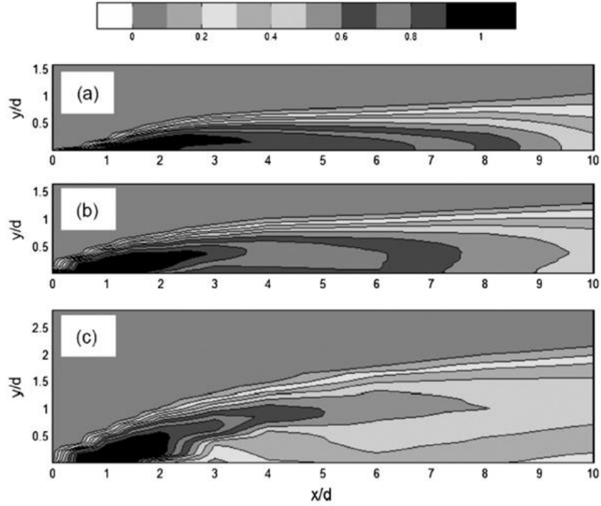
Figure 22: Overall effectiveness along the centerline of attached (a), reattached (b), and detached (c) coolant jet [30]
