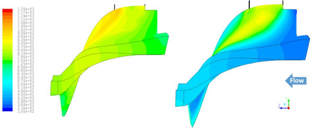
Figure 28: Surface temperature distribution on the solid vane (left) and cooled vane with internal plug (right) [6]
