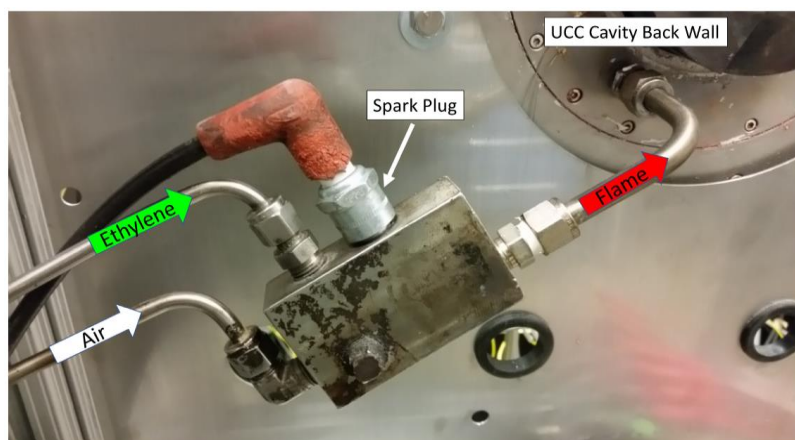
Figure 49: UCC ignition system [33]
