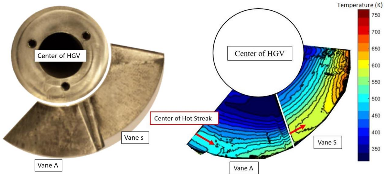
Figure 73: HG hardware of Vanes A and S (left) and IR image (right) at Case 2
