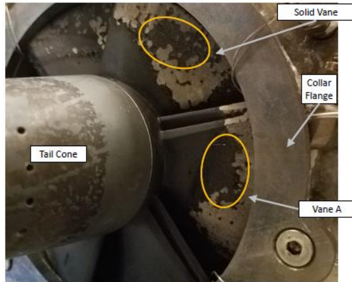
Figure 34: Paint failure on HGV trailing surface [33]
