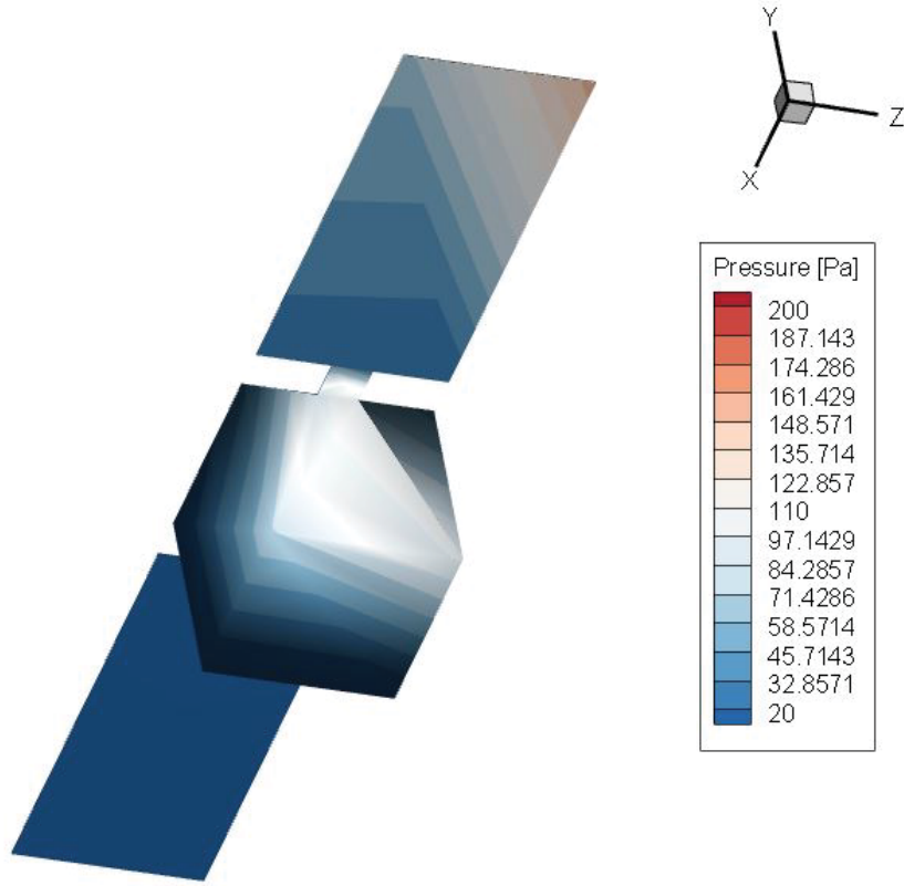
Figure 22. Pressure Distribution: 90 km, Flow Positive X-Direction
