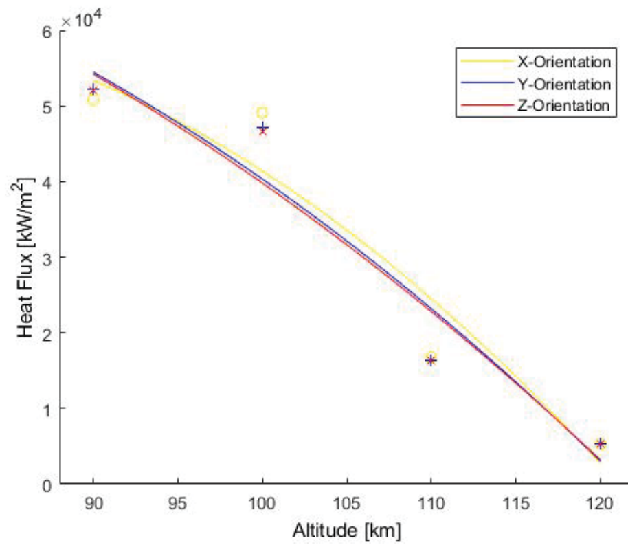
Figure 30. Maximum SPARTA Skip Perigee Heat Flux
