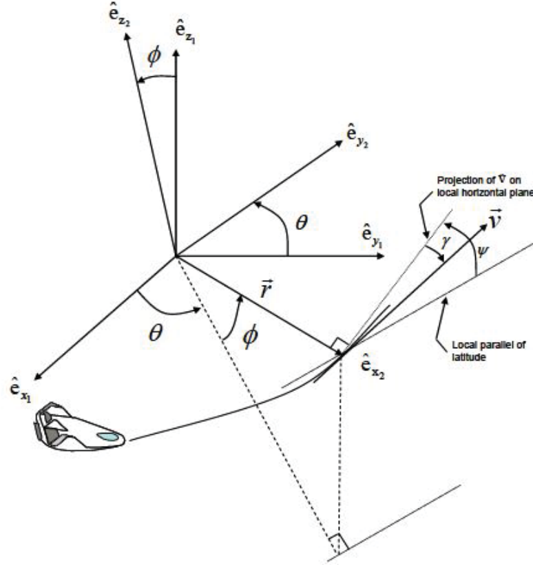
Figure 16. Vehicle Pointing System [6]
