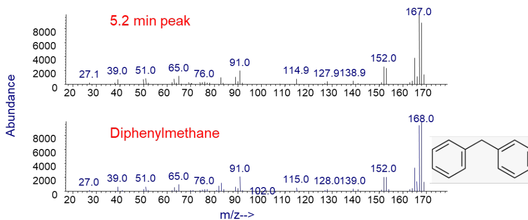
Fig. D-10 Mass spectrum and library search match (with structure) of 5.2-min peak from 750 °C pyrolysis of phenolic resin
