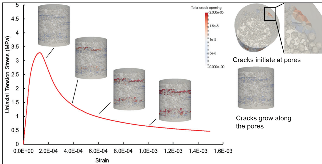
Figure 9. The stress/strain curve and corresponding snapshots of crack opening on the specimens with mesopores under uniaxial tension.
