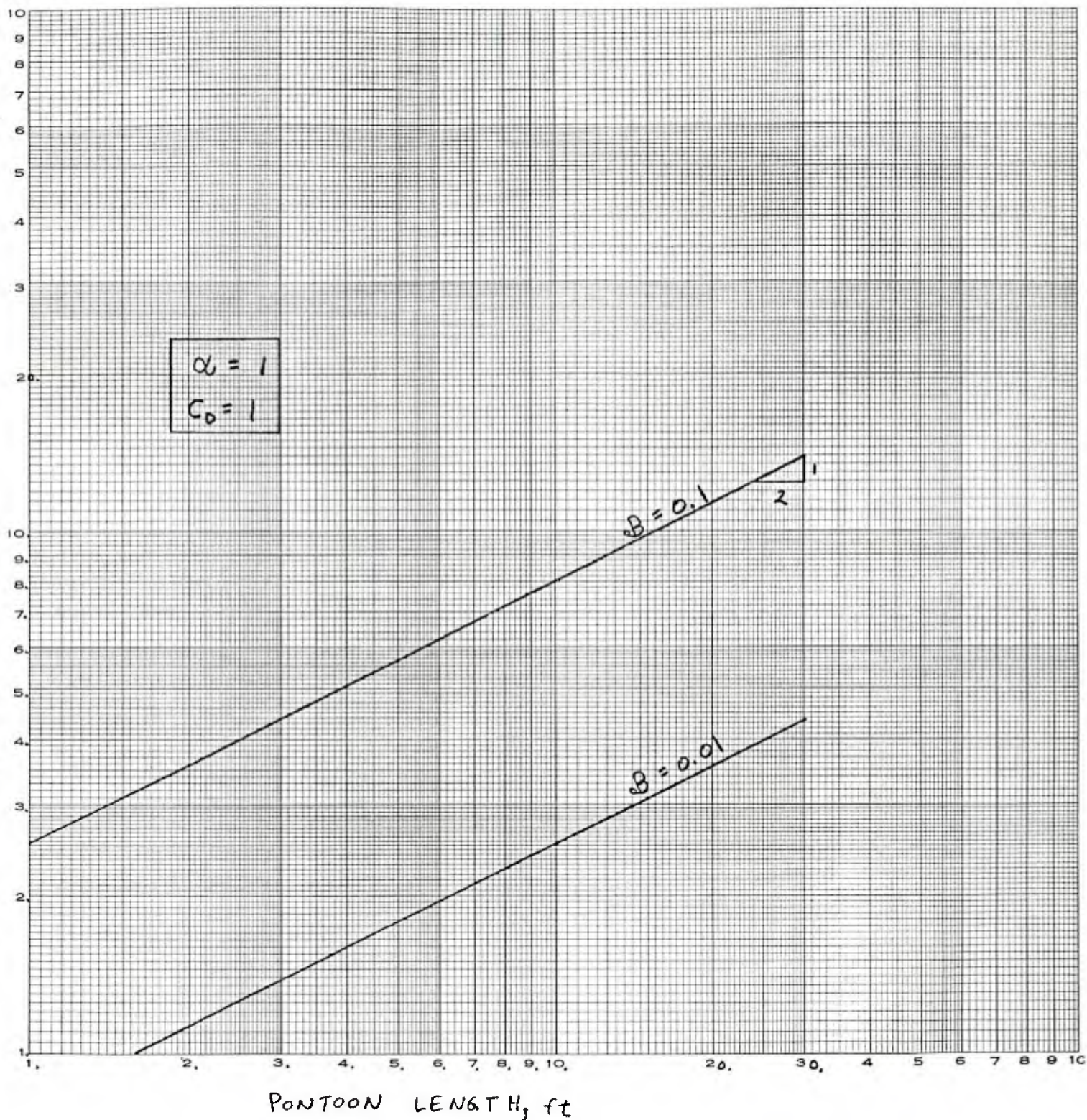
FIGURE 1. VARIATION OF ASCENT VELOCITY WITH PONTOON LENGTH AND BUOYANCY RATIO.
