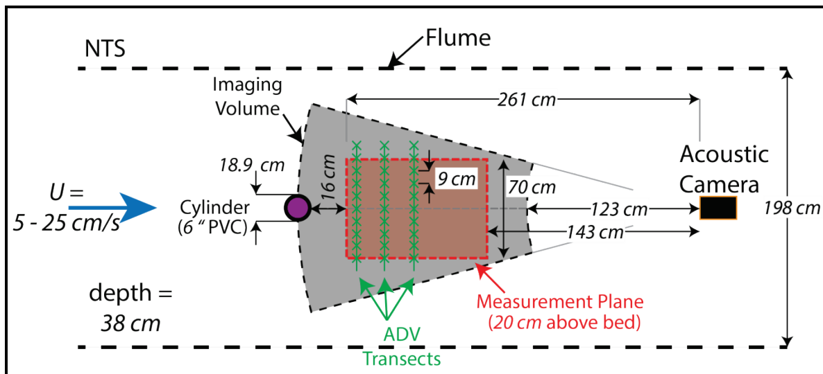
Figure 5. Diagram of the experimental setup.
