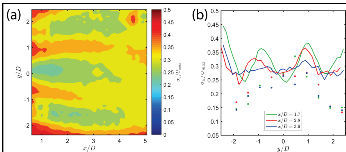
Figure 8. (a) Standard deviation of downstream velocity ( \sigma_u ) from the acoustic camera and (b) comparison of standard deviation of downstream velocity between ADV cross sections (dots) and acoustic camera cross sections (lines).
