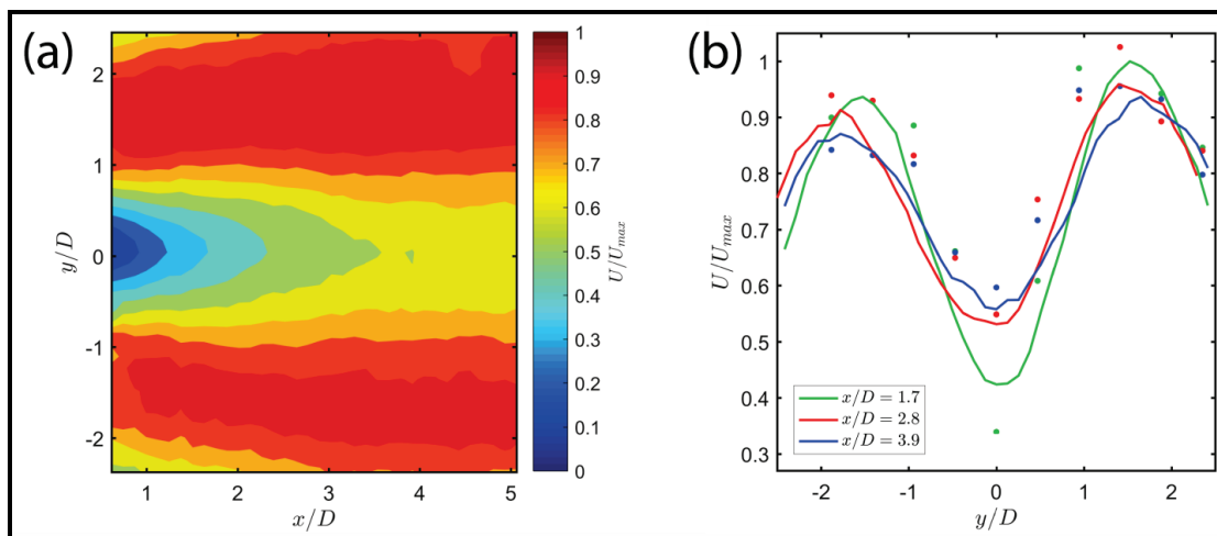
Figure 6. (a) Mean downstream velocity ( U ) from the acoustic camera and (b) comparison of mean downstream velocity between ADV cross sections (dots) and acoustic camera cross sections (lines).
