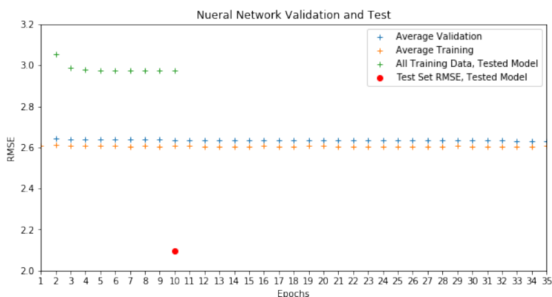
Figure 22. This figure clips the values of the first epoch to focus on the convergence of the RMSE over training iterations. The final model was trained on the entire training set for ten epochs. The resulting RMSE on the test set is shown in red.
