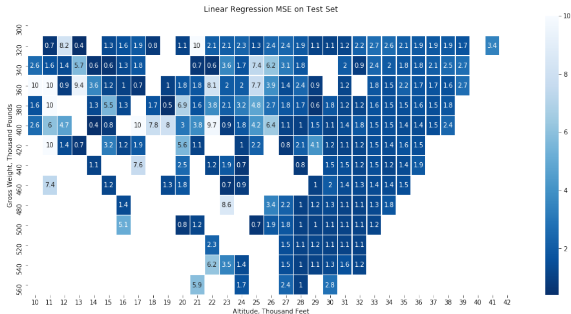
Figure 23. Linear Regression Test MSE
