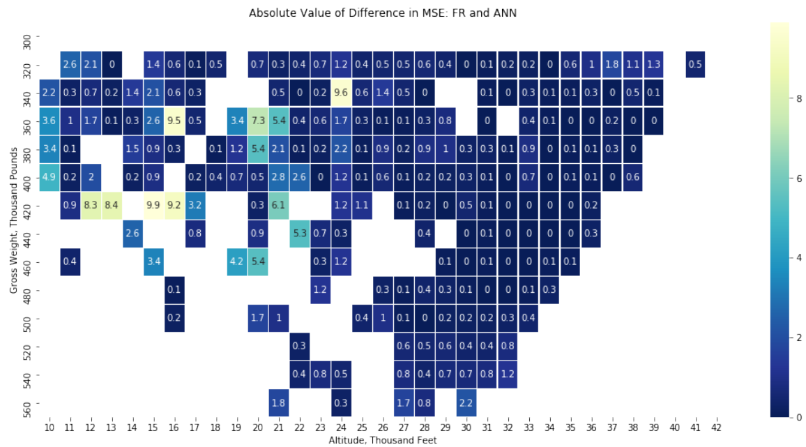
Figure 27. The absolute difference in performance on the test between forest regression and ANN. A value of ten indicates a MSE difference of ten or greater.
