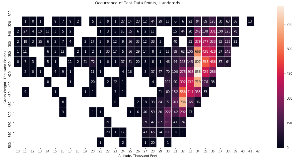
Figure 17. How many data points, in hundreds are closest to a given gross weight and altitude in the test data used. Areas where there were no data points were are white. Areas that show 0 are areas where there are more than 30 data samples but less than 100.
