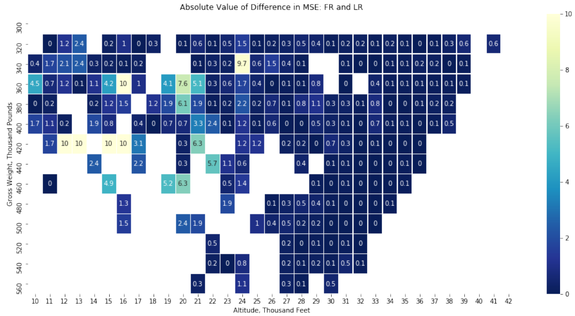
Figure 26. The absolute difference in performance on the test between forest regression and linear regression. A value of ten indicates a MSE difference of ten or greater.
